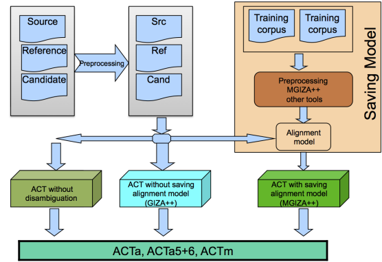
Figure 1: ACT architecture
