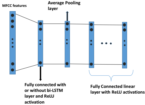
Fig. 1: The neural network architecture of triplet-loss approach for text-dependent SV.
