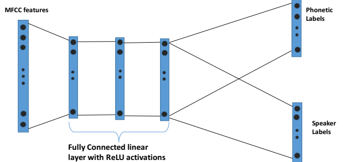
Fig. 2: Multi-task learning for Random-digit task.
