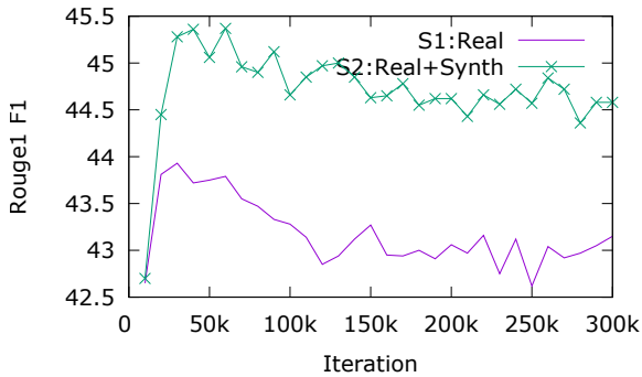
Figure 3: Learning curves in terms of Rouge1 F1 (R1_F1) Score on dev set.
