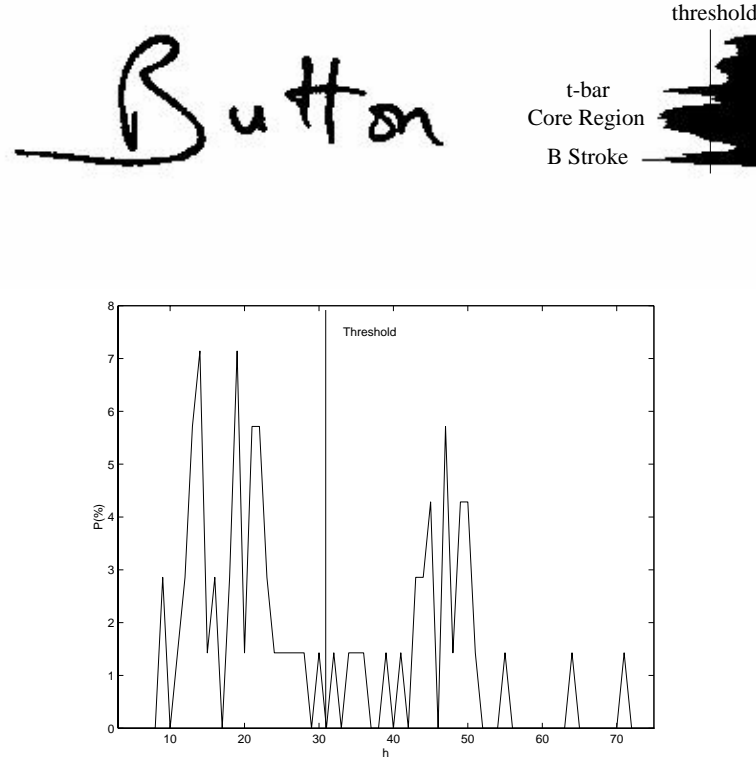
Figure 3: Peaks determined by horizontal strokes are evident in the density histogram (upper figure). In the density probability distribution (lower graphic), the density values of the peaks have small probability. Their influence is negligible and they do not influence the calculation of the threshold.
