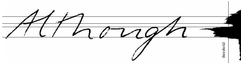
Figure 2: The proposed core region detection method: the density threshold gives a first rough estimate of the core region. A high density region is located in the ascender area, but can be discarded by simply selecting the high density region containing the highest number of foreground pixels.
