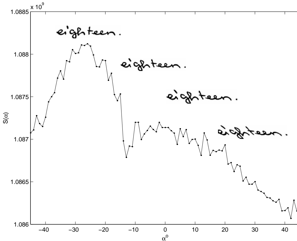
Figure 5: Deslanting algorithm. The plot of S(\alpha) shows a high peak in correspondence of the deslanted image. For high values of \alpha , when the image is strongly deformed, the value of S(\alpha) becomes lower.
