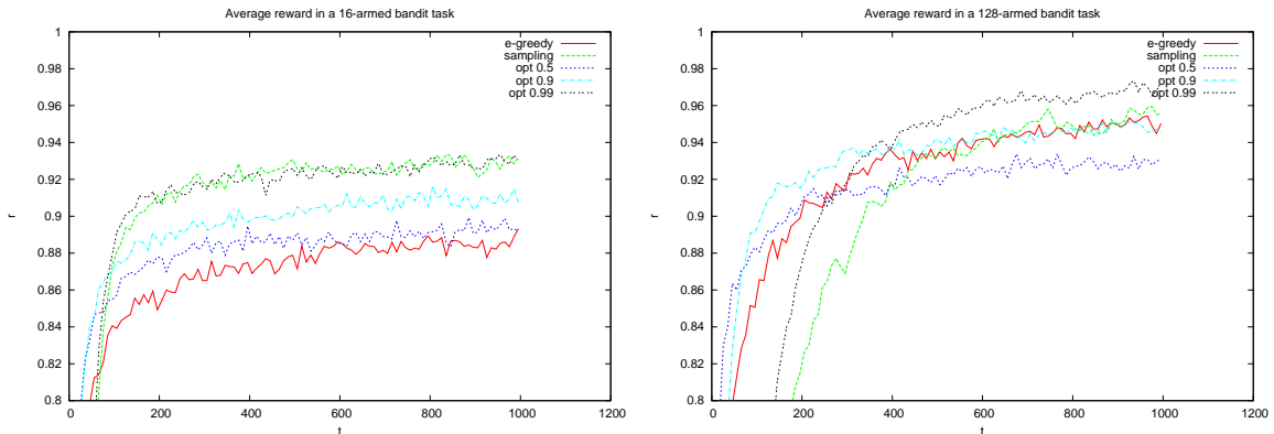
Figure 1: Average reward in an multi-armed bandit task averaged over 1,000 experiments, smoothed with a moving average over 10 time-steps. Results are shown for \epsilon -greedy ( e-greedy ), sampling-greedy ( sampling ) and Alg. 2 ( opt ) with \gamma \in \{0.5, 0.9, 0.99\} .
