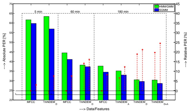
Figure 1: PER results: HMM/GMM and SGMM systems trained using MFCC and posterior-based (Tandem) features evaluated on Afrikaans. Relative improvements of each system (red dashed lines measured on the right vertical axis) are given with respect to HMM/GMMs trained on MFCCs (for given training scenario).
