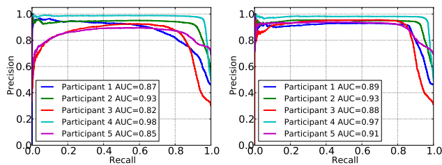
Fig. 16 Automatic gaze coding precision-recall curves obtained without alignment (left) and using alignment (right).
