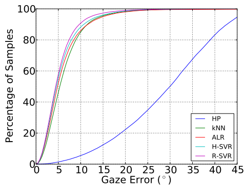
Fig. 8 Recall-error curve obtained for each of the gaze estimation methods. FT target, person-specific model ( PS ), minimal head pose variations ( SP ).
