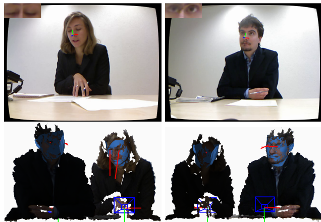
Fig. 15 Gaze coding in a dyadic interaction. Top: original RGB frames. Bottom: 3D rendering of the composed 3D scene from two viewpoints, including the estimated head pose and 3D gaze direction.
