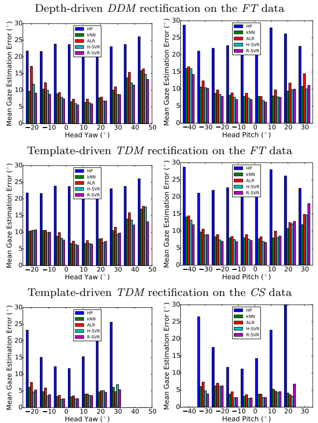
Fig. 12 Gaze error distribution for the right eye in function of the head pose for the FT and CS cases and different pose-rectification rendering methods.
