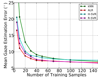
Fig. 10 Mean angular error vs. number of training samples. Conditions: FT target, person-specific model ( PS ), minimal head pose variations ( SP ).
