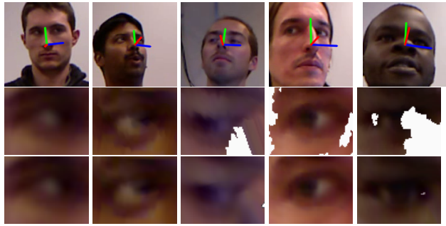
Fig. 6 EYEDIAP samples and pose-rectified images. Each column correspond to one data sample. Per row we show i) the head pose, showing a region of 140 \times 140 pixels from the RGB frame; ii) \mathbf{I}^R images generated from the depth data ( DDM ); iii) \mathbf{I}^R images generated from the template data ( TDM ). The first three columns correspond to sessions involving the FT target, whereas the last two correspond to samples for the CS target.
