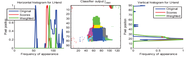
Figure 3: Body part histogram example. Left and right: m_{l,v}^{\vec{}} and m_{l,h}^{\vec{}} for the left hand. Center: classifier output. The confidence weighting helps to maintain the detection peak in the right position. Best viewed in color.
