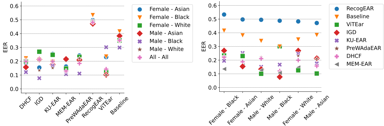
Figure 4. Comparison of differential performance due to demographics at the EER operating point. The left graph shows the performance differentials of the tested models w.r.t. different demographic sub-groups and the right graph shows the performance spread for each sub-group across all models. The figure is best viewed in color.
