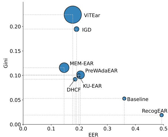
Figure 2. Comparison of the verification performance (EER) vs. bias behavior (Gini). The surface area of the circles represents the number of trainable parameters. For reference, the smallest model (Baseline) has around 11.7M parameters and the largest (ViTEar) has 304.9M. An ideal method would be located at the origin of the coordinate systems.
