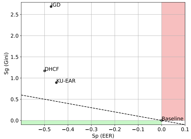
Figure 5. Comparison of changes in verification performance S_p (EER) and demographic bias S_g compared to the baseline. Ideally, the tested models would fall into the bottom left quadrant (marked with green), where both verification errors and bias are decreased. The worst scenario is within the top right quadrant (marked with red), where both the error and bias increase. All track 2 approaches are somewhere in between, i.e., they did not reduce bias, but they did improve verification performance.
