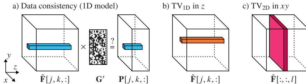
Fig. 3. Regularization with TV_{1+2} implements 3D prior constraints while keeping efficient computations using a parallel implementation. (a) Data consistency relies on the 1D forward model. (b) TV_{1D} regularization along the compression axis is tuned separately to account for anisotropy in the volume. (c) Isotropic TV_{2D} on xy sections allows information sharing between the many 1D problems.
