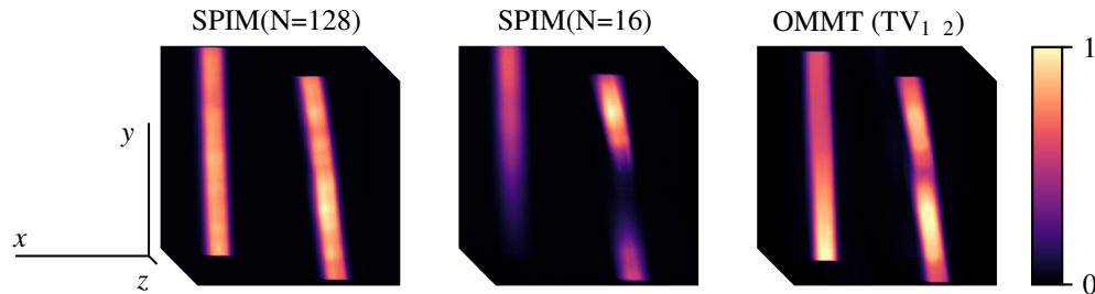
Fig. 9. OMMT reconstruction of fluorescent textile fibres and comparison to undersampled SPIM, with a larger depth span of 800\ \mu\text{m} . Information located between sampled planes is missing in the undersampled SPIM volume, where no gaps are present in the \text{TV}_{1+2} image. Views use mean intensity projection, and axes are 100\ \mu\text{m} scale bars.
