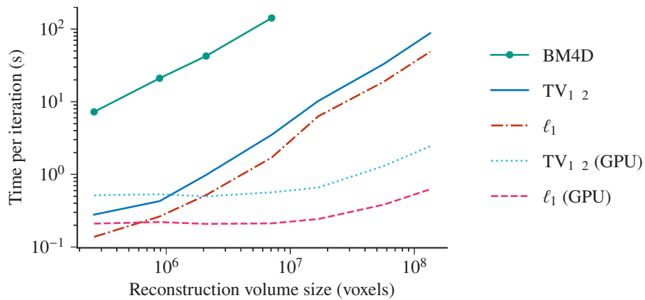
Fig. 7. Average time per iteration of our ADMM optimization loop for different regularization priors. BM4D is not realistically useable to reconstruct big images, but both TV_{1+2} and \ell_1 are fast enough to be applied to real size experimental data. This is particularly true with the 30\times speed-up when running with GPU acceleration. See Table 2 for detailed values.
