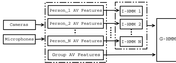
Figure 1: Framework overview
