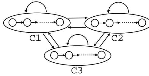
Figure 2: Fully connected HMM topology
