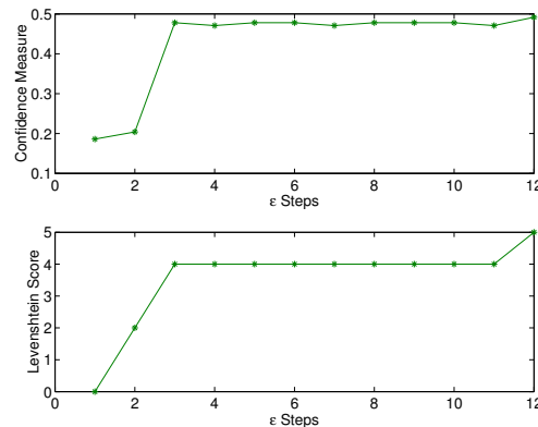
Figure 6.4. A case where the baseform pronunciation of word keeble in PhoneBook database uttered by a female speaker doesnot match well with the acoustic observation. The inference was done with acoustic models of system-app-p .
