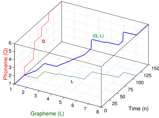
Figure 7.3. 3D Viterbi decoding in phoneme-grapheme based ASR.
