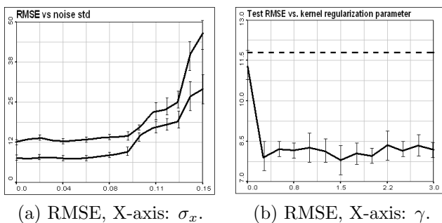
Fig. 2. Spiral data experimental results.
