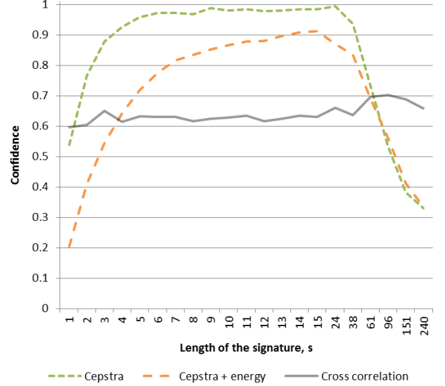
Figure 3. Confidence versus signature / test segment length.
