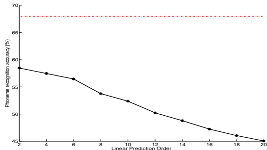
Figure 2: Phoneme recognition: The x-axis shows the LP order while the y-axis shows the phoneme accuracy in (%).
