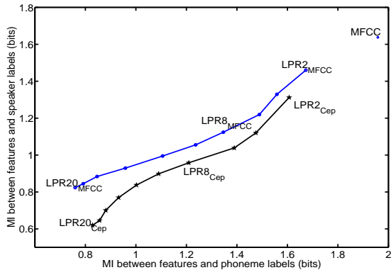
Figure 1: Plot showing MI between residual features and phonemes vs MI between residual features and speakers. LPRx denotes residual with prediction order x . The subscript denotes real-cepstrum or MFCC. Lone point denotes baseline MFCC.
