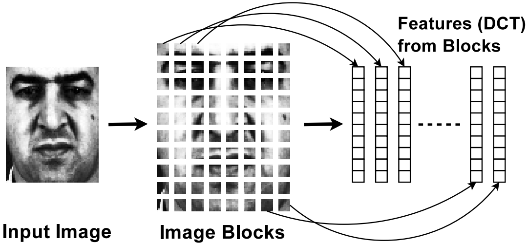
Figure 1: The process of extracting DCT block features from a geometrically normalized image.
