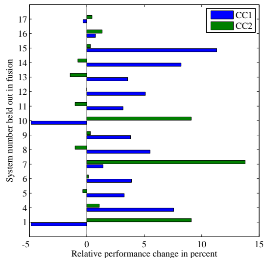
Figure 1: Analysis of excluding one system at a time in fusion using Focal and employing compound log-likelihood ratio [34] for P_{\text{known}} = 0.5 . Using the full ensemble of classifiers results in actual C_{\text{primary}} of 0.3959 and 0.2836 for first two common conditions (CC1 and CC2) respectively in SRE'12 for the pooled scores of males and females. A positive relative change indicates increased actual C_{\text{primary}} by excluding a system in fusion resulting in fusion performance drop. Systems number 2 and 3 are not considered for this analysis.
