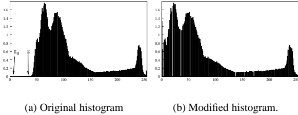
Figure 1: Histogram modification.
