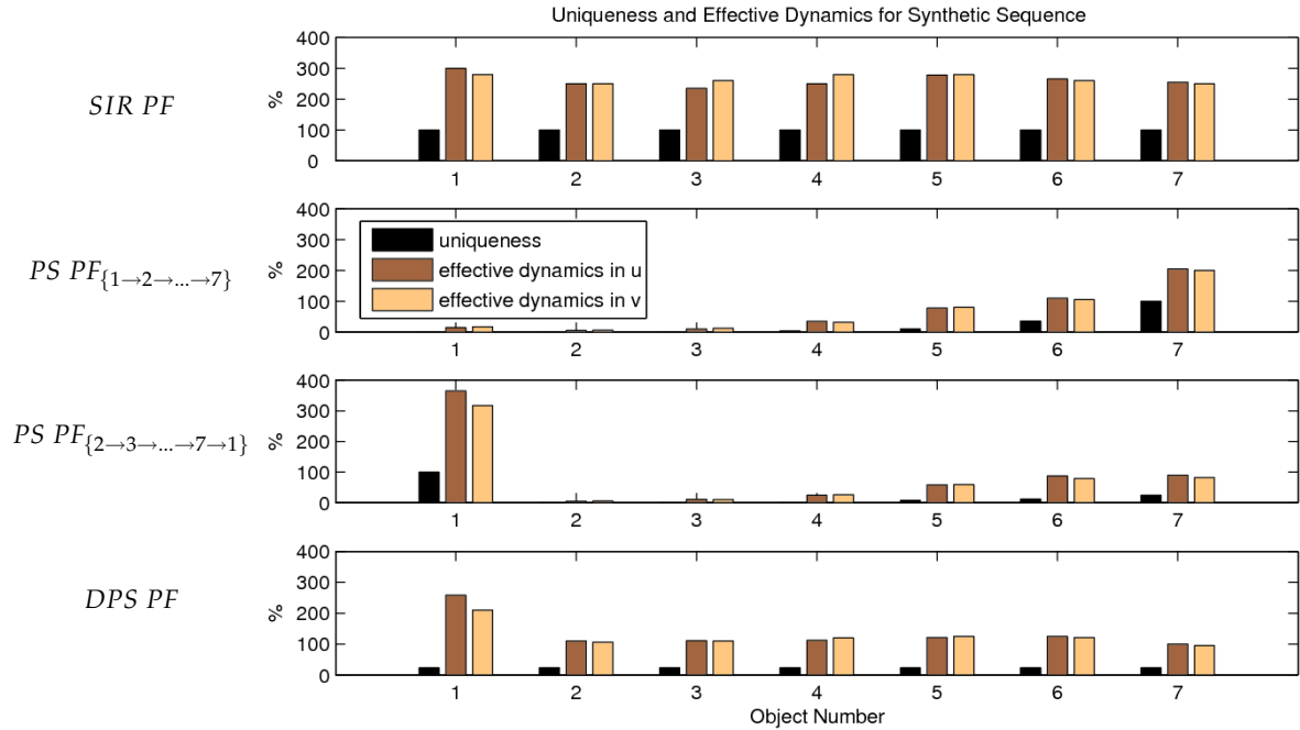
Figure 4.11. Uniqueness and effective dynamics for the 7 objects in the synthetic sequence (50 runs, \lambda = 20 , N = 300 ). The SIR PF (top) does not suffer any impoverishment effects. In contrast, the PS PF suffers impoverishment effects according to the ordering, as seen for the middle plots. The distributed partitioned sampling particle filter (DPS PF) described in Section 4.3 fairly spreads the impoverishment effects among the objects, as seen in the bottom plot.
