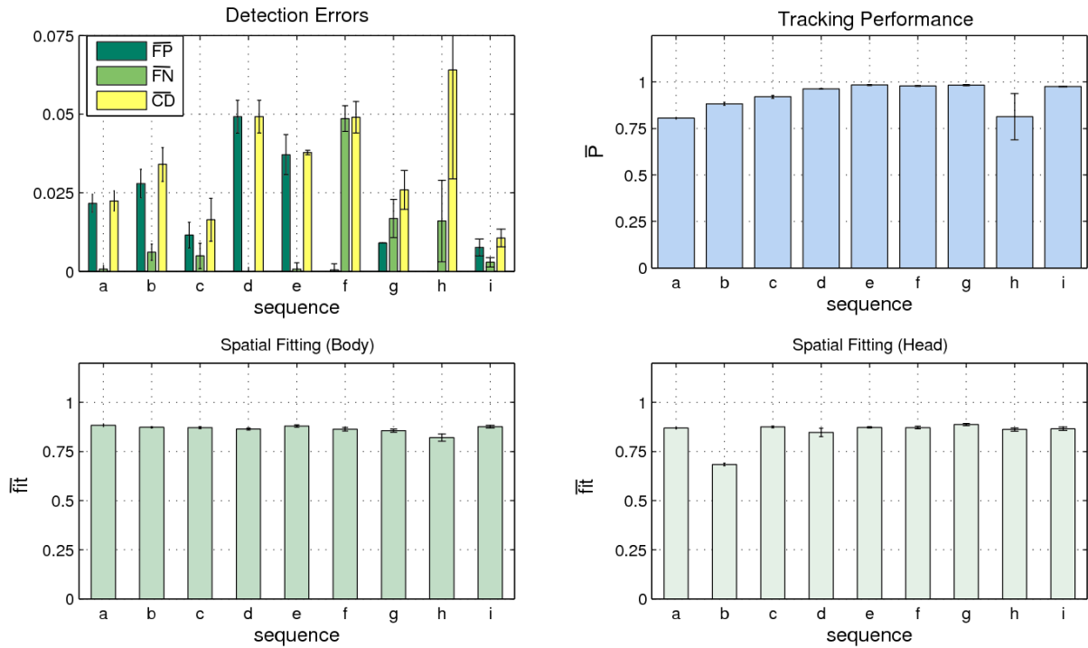
Figure 7.9. Multi-person head and body tracking results. The detection performance plot in the upper left measures the ability of the model to estimate the correct number and placement of people in the scene. Measures shown include the normalized false positive ( \overline{FP} ) and false negative ( \overline{FN} ) error rates (per person, per frame), and the counting distance ( \overline{CD} ) (near-zero values are good, see Chapter 3). The tracking performance plot in the upper right measures the ability of the model to persistently track people over time. The purity measure \bar{P} measures the consistency with which the ground truths and estimates were properly identified. \bar{P} values near 1 indicate good performance. The lower plots show the spatial fitting results (how well the tracker bounding boxes fit the ground truth) for the body and the head over the nine sequences. Overlap between the estimate and ground truth are measured by \overline{fit} . A value of 1 indicates a perfect fit, a value of zero indicates no overlap. In each plot, the standard deviation is represented by error bars (cases where no error bar is visible indicates standard deviation = 0).
