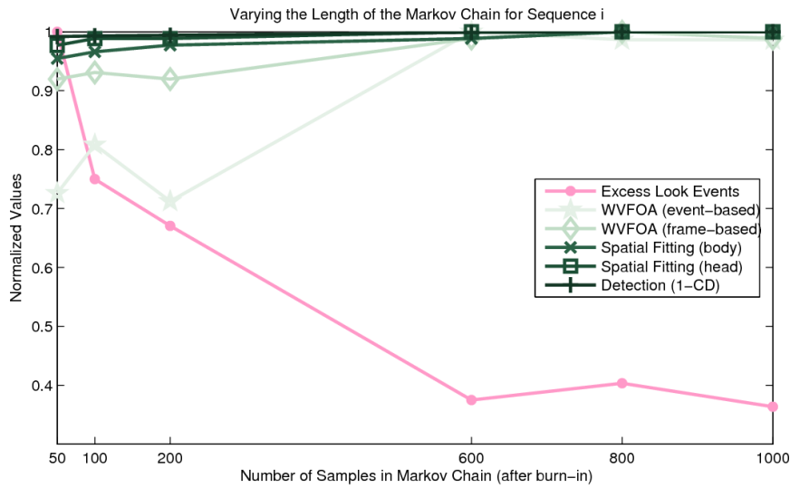
Figure 7.11. Varying the number of samples in the Markov Chain. As more samples used, various performance gauges increase, as seen here for sequence i . Excess (false alarm) look events detected by the system drop as more samples are added (shown in pink), the WVFOA recognition improves (both event and frame based), spatial fitting for the body and head improves, and detection performance increases (as measured by 1 - \overline{CD} ). Note that the measures have been normalized to appear on the same axis.
