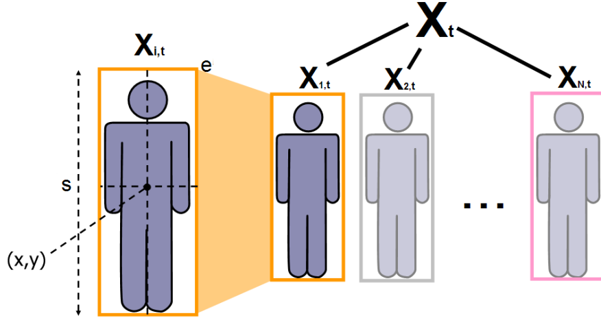
Figure 5.14. The state-space for the RJMCMC PF. The joint multi-person state, X_t consists of an arbitrary number of people X_{i,t} . Each person is modeled as a bounding box with parameters for the location (x, y) , height scale s , and eccentricity e .
