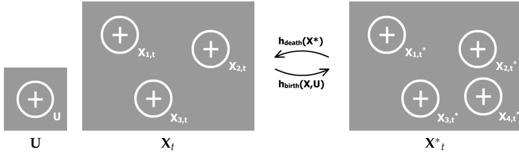
Figure 5.8. Birth and death moves. The birth move makes the transition from an initial state (\mathbf{X}_t, \mathbf{U}) to a proposed state \mathbf{X}_t^* by adding a new object ( \mathbf{X}_{4,t}^* = \mathbf{U} ) to the multi-object configuration, keeping all other objects fixed. To revert to the original state, the death move is applied to \mathbf{X}_t^* .
