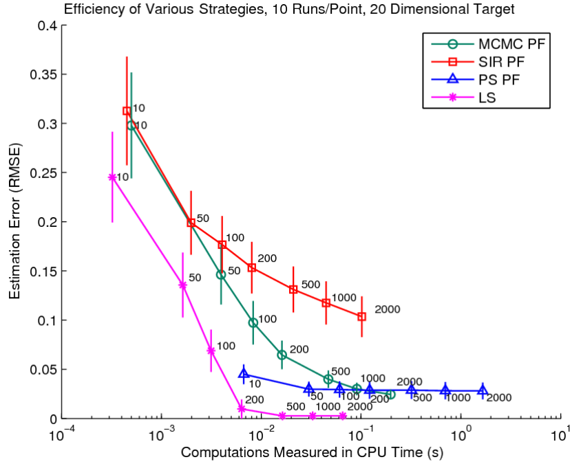
Figure 3.13. Efficiency and computational cost of various strategies.
