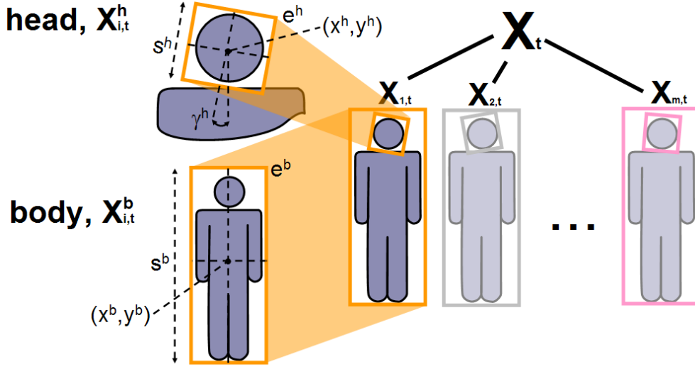
Figure 6.2. The state-space for the RJMCMC PF head tracker. The joint multi-person state, \mathbf{X}_t consists of an arbitrary number of people \mathbf{X}_{i,t} , each containing a body \mathbf{X}_{i,t}^b and head \mathbf{X}_{i,t}^h component. The body is modeled as a bounding box with parameters for the location (x^b, y^b) , height scale s^b , and eccentricity e^b . The head location \mathbf{X}^h has similar parameters for location (x^h, y^h) , height s^h , and eccentricity e^h , as well as in-plane rotation \gamma^h .
