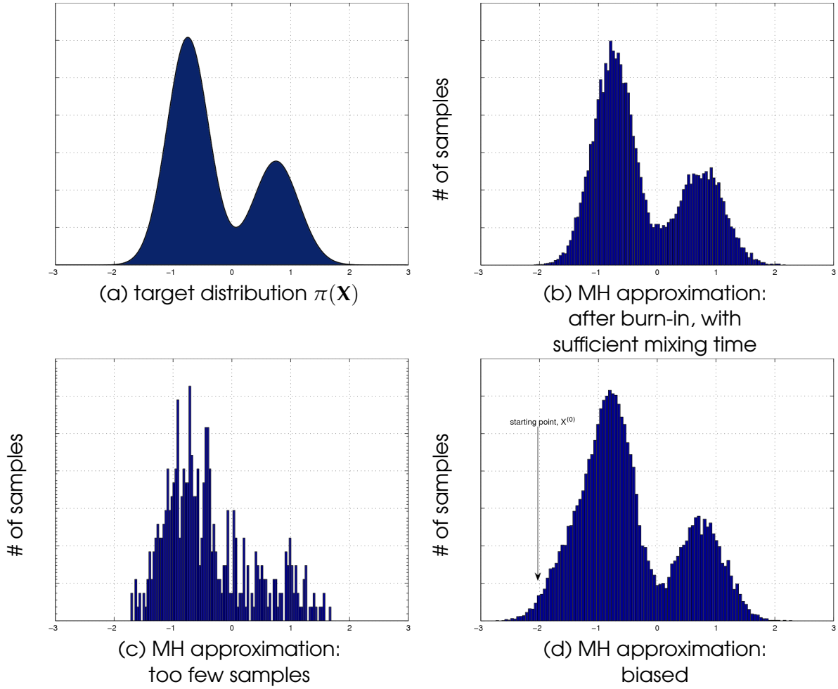
Figure 5.3. Mixing time and bias concerns in MH. In (a), a target distribution \pi(\mathbf{X}) is shown. In (b), we show the Metropolis-Hastings approximation of the target distribution given sufficient mixing time, and after removing the N_B burn-in samples (starting at \mathbf{X}^{(0)} = 0 ). In (c), we see the effect of an insufficient mixing time, and in (d) we see the effect of not removing the N_B burn-in samples, when starting at \mathbf{X}^{(0)} = -2 (exaggerated in this illustration).
