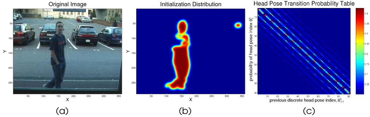
Figure 7.3. Initialization distribution and head-pose transition probability table. The initialization distribution in (b) determines where to place a new person in the scene by applying a Gaussian smoothing filter to the foreground segmentation of the original image (a). The head-pose transition probability table in (c) shows how the head-pose exemplars switch from the previous to current time step p(\theta_t^h | \theta_{t-1}^h) . Visible lines show that transitions are most probable between similar poses.
