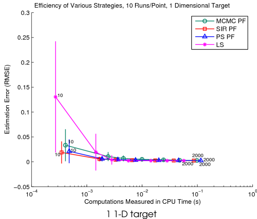
Figure A.1. Effectiveness of various search strategies for 1 target object.
