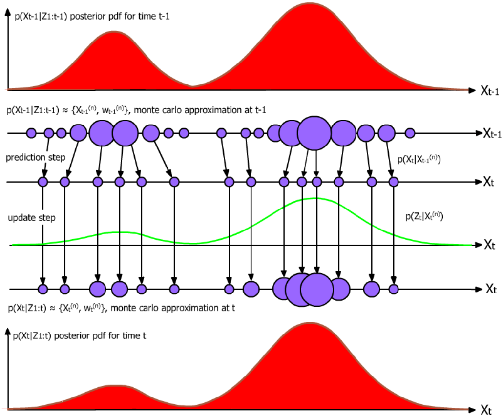
Figure 2.14. Sequential Importance Resampling (SIR) Particle Filter. Given a set of weighted samples which approximates the t - 1 posterior distribution p(\mathbf{X}_{t-1}|\mathbf{Z}_{1:t-1}) \approx \{\mathbf{X}_{t-1}^{(n)}, w_{t-1}^{(n)}\}_{n=1}^N , the SIR particle filter estimates the posterior distribution at time t in two steps, prediction and update . In the prediction step, N samples are drawn from the previous distribution and the dynamic process is applied. In the update step, the samples are weighted according to the observation likelihood function. The result is a set of weighted samples which approximates the current distribution p(\mathbf{X}_t|\mathbf{Z}_{1:t}) \approx \{\mathbf{X}_t^{(n)}, w_t^{(n)}\}_{n=1}^N .
