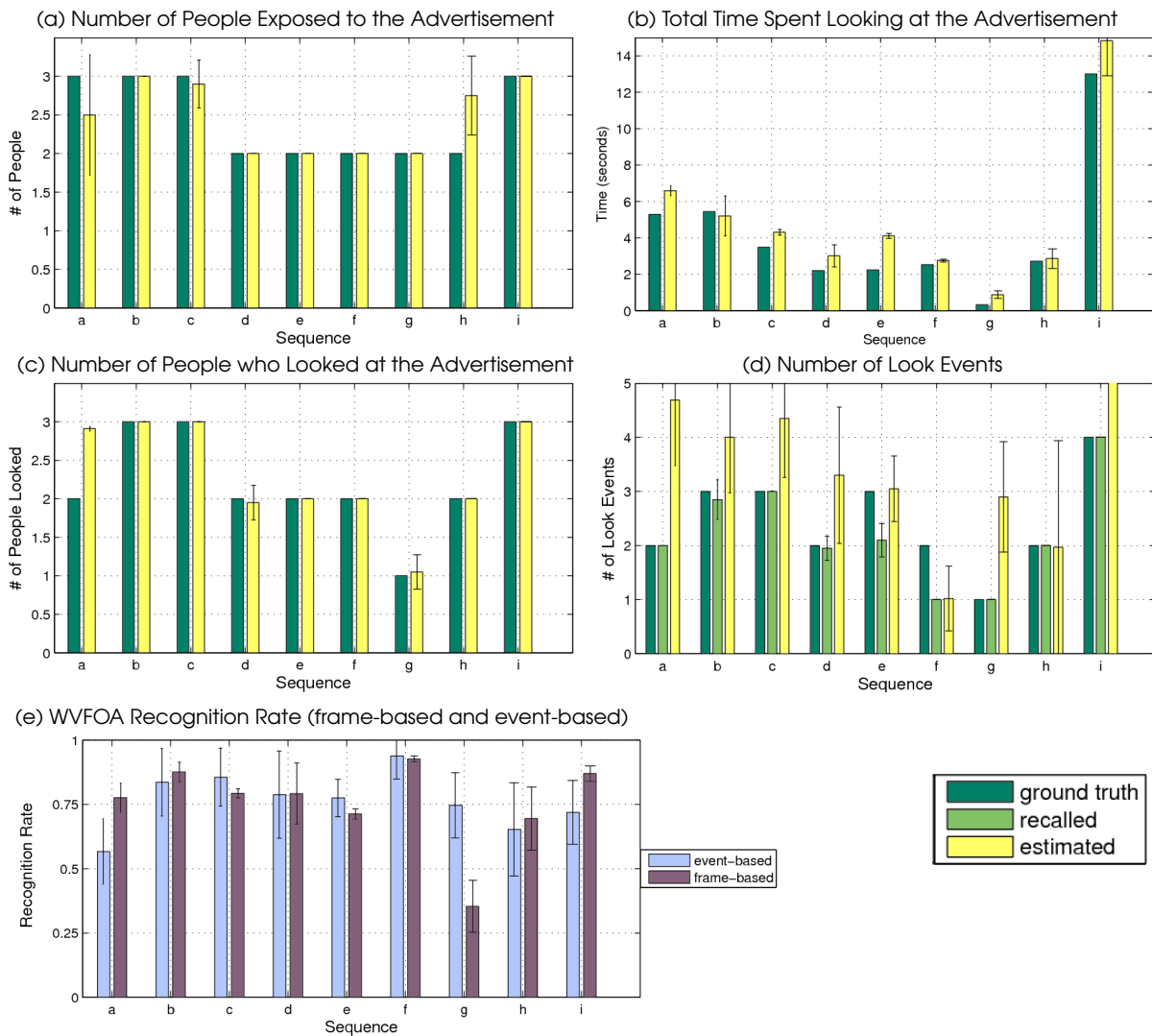
Figure 7.10. Ad application results. Plot (a) shows the results for estimating the number of people exposed to the advertisement for each sequence. Plot (b) shows the results for estimating the amount of time people spent looking at the advertisement for each sequence. Plot (c) shows the results for estimating the number of people who looked at the advertisement. Plot (d) shows the results for estimating the number of “look events” for the nine sequences. Plot (e) shows the overall recognition rate of focused and unfocused states (calculated based on events and based on frame counts). For plots (a) - (d), the ground truth appears in dark green and the estimated value in yellow.
