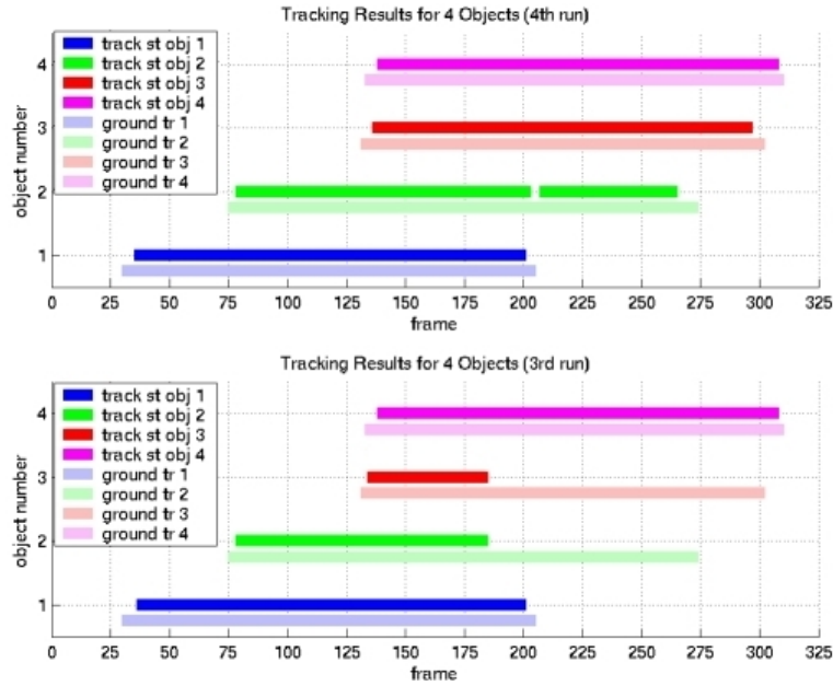
Figure 5.15. Tracking results from seq4 . In the plots above, the track state \tau_j (darker colored bars) and \mathcal{GT} presence (lighter colored bars) are plotted for each of the objects ( j ) present in seq4 . The top plot shows the results for an experimental run where X_2 temporarily loses tracking when occluded by X_4 (frames 201–206). The bottom plot shows the results for an experimental run where X_2 and X_3 mistakenly swap identities at frame 185, though both objects were still detected . Delays in tracking \mathcal{GT} s as they enter the scene are apparent, as the track states are typically of shorter duration than the \mathcal{GT} presence.
