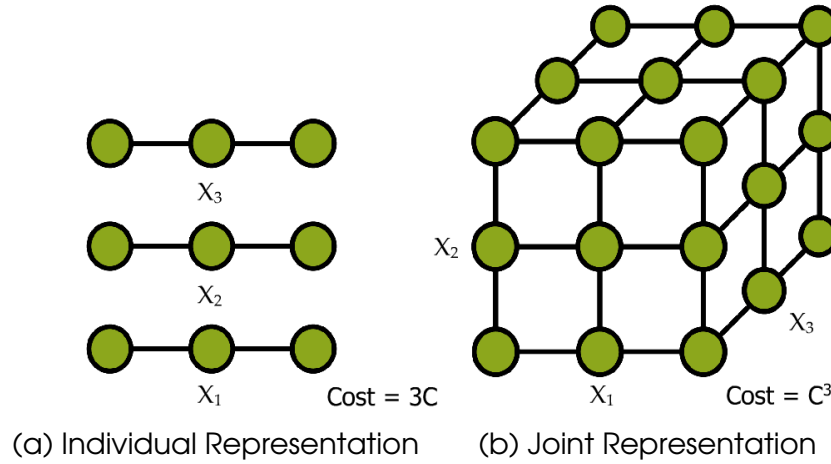
Figure 2.16. The dimensionality curse of joint state spaces. The search space \mathcal{X}_i for an individual object is represented by a set of three circles. If the cost \mathcal{C} associated with searching for a solution to the single object tracking problem is roughly proportional to the size of the search space, \mathcal{C} \propto \mathcal{X}_i , the cost of searching a joint representation of multiple objects is \mathcal{C}^m , whereas searching for each object independently, the cost is m\mathcal{C} .
