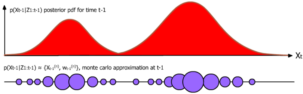
Figure 2.13. The Monte Carlo approximation. The posterior pdf of Equation 2.3 shown in red for the previous time step t - 1 is approximated by a set of N weighted samples \{(\mathbf{X}_{t-1}^{(n)}, w_{t-1}^{(n)})\}, n = 1, \dots, N\} in the Monte Carlo approximation (shown as purple circles).
