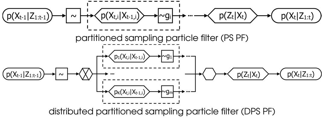
Figure 4.12. PS PF and DPS PF block diagrams. The top diagram shows the PS PF process: the prior, resampling step ( \sim ), partitioned sampling (marked by the dashed box), likelihood, and posterior. In the bottom diagram, DPS PF breaks the sample set into K components, each with a different PS ordering, and reassembles the components.
