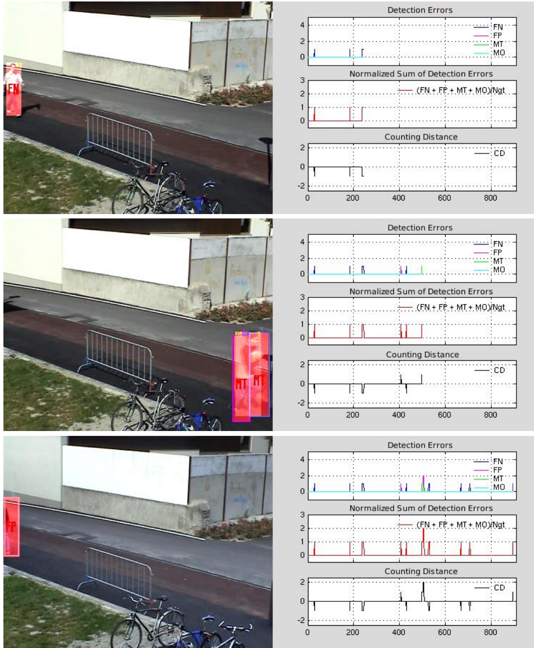
Figure 3.6. Detection evaluation of a video sequence. Detection measures are plotted for a sequence of 908 frames where the task is to track pedestrians ( t_C = 0.33 and t_O = 0.10 ). In each row, three plots on the right show the detection measures (vertical axis) over the course of the sequence (indicated by frame number on the horizontal axis). The top plot shows incidents of the detection errors (FN, FP, MT, and MO). The middle plot shows a sum of the detection errors normalized by the number of \mathcal{GT} s appearing in the frame. The bottom plot shows the counting distance, CD. For more details, refer to the text.
