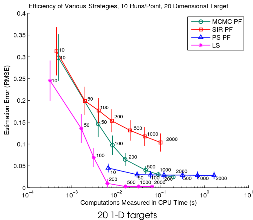
Figure A.3. Effectiveness of various search strategies for 10 and 20 target objects.
