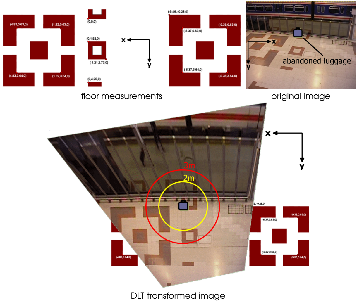
Figure 8.10. Registration and testing for alarm conditions. ( upper left ) The calibration information from the floor pattern provided by PETS is shown. ( upper right ) A bag location is shown in the image plane. ( bottom ) The bag location on the floor plane computed via the DLT, along with the warning and alarm radii denoted by yellow and red circles, respectively. Using the DLT, the bag owners coordinates in the image plane can be transformed to the floor plane, where alarm conditions can be tested by computing the Euclidean distance to the bag.
