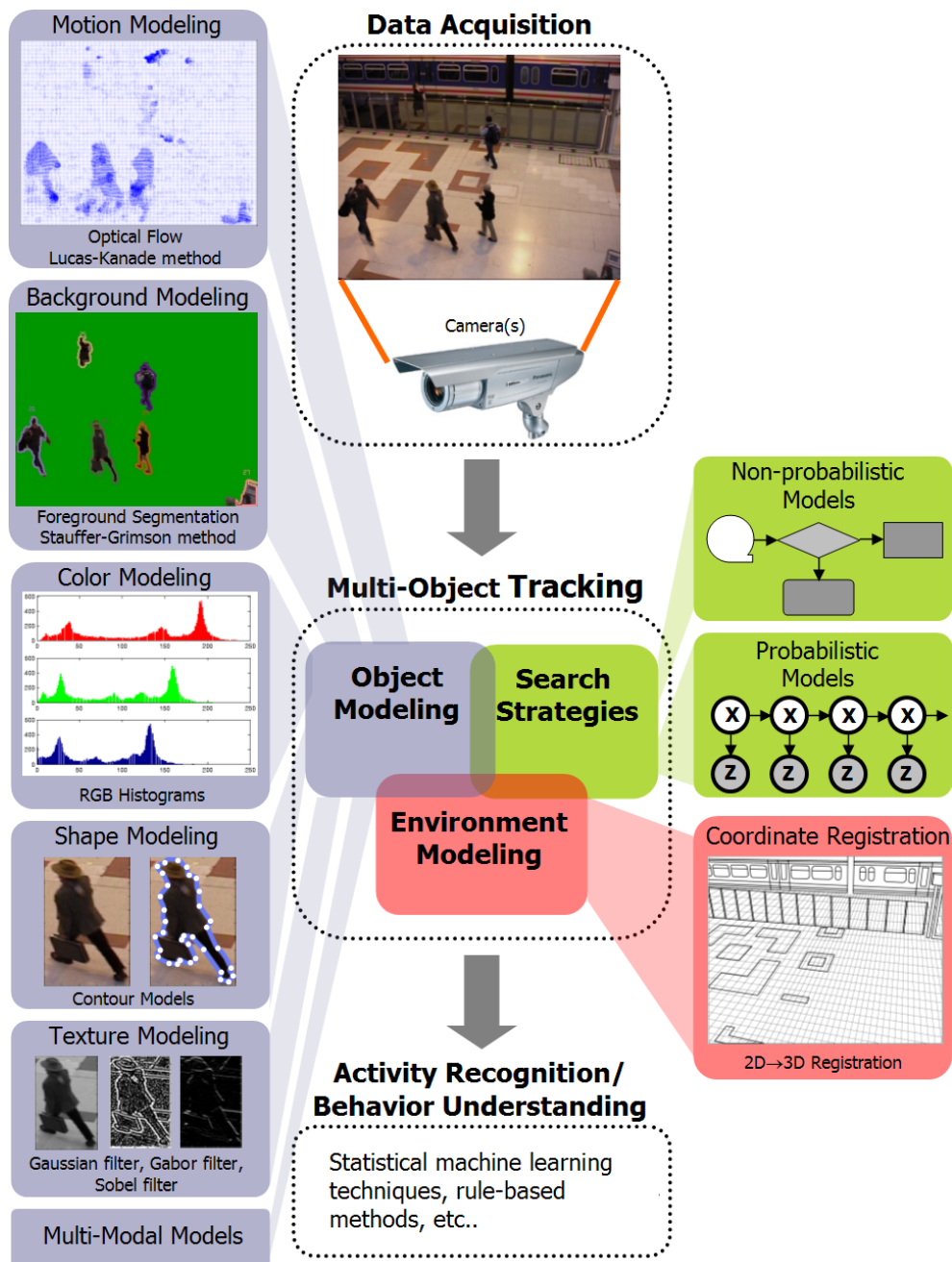
Figure 2.7. The multi-object tracking and activity recognition framework. The problem of multi-object tracking and activity recognition is formulated as three phases: data acquisition, multi-object tracking, and activity recognition. Video data is passed from the data acquisition phase to the multi-object tracking phase, which is comprised of three elements: object modeling, search strategies, and environment modeling. There is often considerable overlap between these elements. Typically, the results of the tracking phase are passed to a final phase responsible for interpreting high-level concepts such as human activity and behavior, though sometimes activity recognition is performed jointly with tracking.
