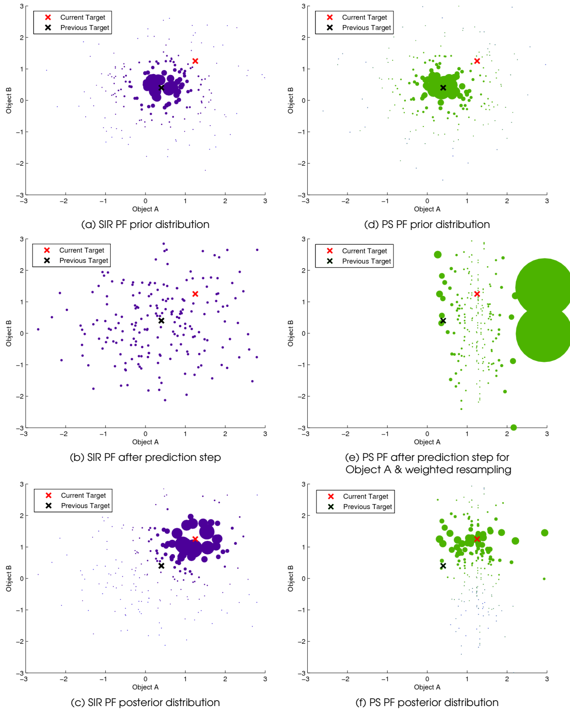
Figure 4.5. SIR PF vs. PS PF. A side-by-side comparison of the operation of the SIR PF and PS PF. Each filter jointly tracks two one-dimensional targets A and B . The joint object location at t - 1 is represented by a black cross, and by a red cross at t . (a) and (d) show the posterior distribution at t - 1 . In (b), the SIR PF prediction step spreads the samples in all directions, while in (e) the PS PF single-object prediction step and weighted resampling concentrates the samples near object A , and re-weights them to preserve the distribution. In (c) and (f), the posterior distributions are shown. Notice that the samples in (c) span the entire plot, while the samples in (f) are more concentrated.
