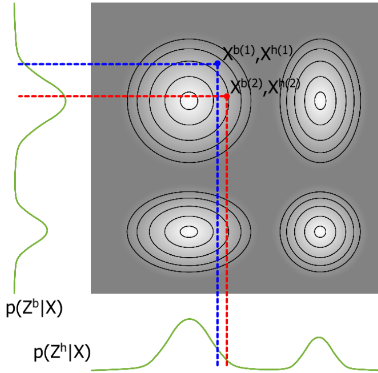
Figure 6.3. Decoupling the update move. The head and body likelihood functions ( p(\mathbf{Z}_t^h | \mathbf{X}_t) and p(\mathbf{Z}_t^b | \mathbf{X}_t) ) are shown in green. The overall likelihood is a product of p(\mathbf{Z}_t^h | \mathbf{X}_t) and p(\mathbf{Z}_t^b | \mathbf{X}_t) , as depicted by the gray surface. Starting at an initial head and body configuration represented by the blue point (\mathbf{x}_t^{b(1)}, \mathbf{x}_t^{h(1)}) the likelihood values might be p(\mathbf{Z}_t^b | \mathbf{x}_t^{(1)}) = 10 and p(\mathbf{Z}_t^h | \mathbf{x}_t^{(1)}) = 100 , giving an overall likelihood of p(\mathbf{Z}_t | \mathbf{x}_t^{(1)}) = 1000 . If a new body and head configuration represented by the red point were proposed (\mathbf{x}_t^{b(2)}, \mathbf{x}_t^{h(2)}) which resulted in a higher overall likelihood p(\mathbf{Z}_t | \mathbf{x}_t^{(2)}) = 5000 (and would thus be accepted and added to the Markov Chain), it is possible for the body configuration to improve while the head configuration worsens ( p(\mathbf{Z}_t^b | \mathbf{x}_t^{(2)}) = 500 and p(\mathbf{Z}_t^h | \mathbf{x}_t^{(2)}) = 10 ). To avoid this situation, we decouple the update move into two separate moves: body update and head update .
