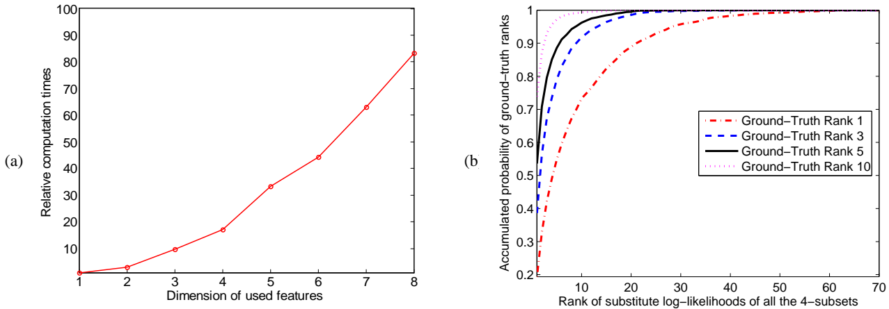
Fig. 1: (a) Relative computation time of LogitBoost classifiers, for different feature sizes. Size one is taken as reference; (b) Grouth-truth ranks of \{L_r(S_{m,i})\} vs. approximated ranks of \{\tilde{L}_r(S_{m,i})\} , for m = 3 .
