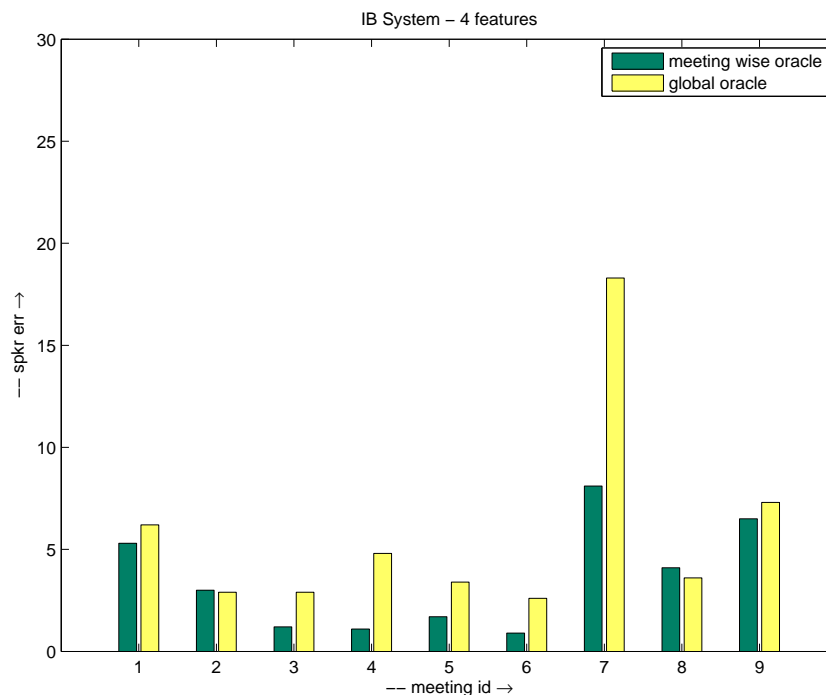
Figure 5.4. Comparison of meeting-wise oracle (feature weights that minimize speaker error for each meeting) performance with the global oracle (same feature weights across all meetings that minimize the overall speaker error) for four feature stream combination with IB system
