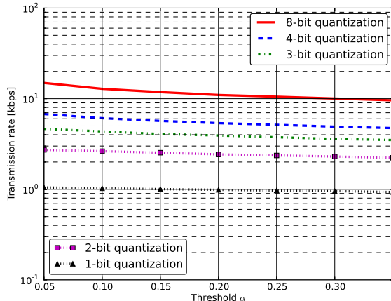
Fig. 3. Estimated transmission rate of different quantization schemes.
