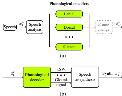
Fig. 1. The phonological vocoder split into (a) encoder and (b) decoder. The encoder runs individual phonological encoders and merges phonological posteriors. The decoder generates speech spectral lines LSPs and source parameters and re-synthesise the speech.
