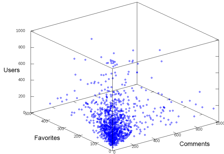
Figure 3.3: Three-dimensional representation of the numbers of favorites and comments, and the unique users that made them for each talk, showing the skewed distribution of user feedback. The number of comments is on the x -axis, the number of favorites is on the y -axis, and the number of unique users that gave feedback is on the z -axis.
