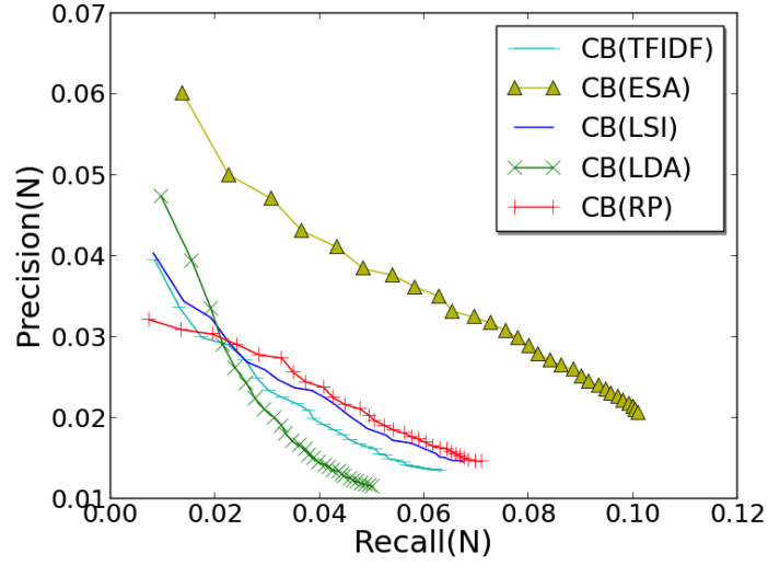
Figure 3.6: Scores of content-based methods in a cold-start setting, in terms of precision and recall at N ( 1 \leq N \leq 30 ) on the held-out set \mathcal{T} . The ESA-based distance outperforms by far all the others, while LSI and RP outperform TF-IDF for most values of N , and LDA outperforms TF-IDF for low values of N (1 to 4).
