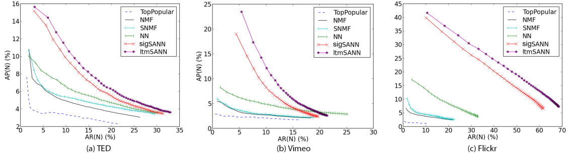
Figure 4.6: Model comparison in terms of average recall at N (horizontally) and average precision at N (vertically), for N from 1 to 50, on the sparse held-out sets . Data points with lower values of N have higher precision and lower recall. The top-scoring curves, upper-right, correspond to the ltmSANN model.
