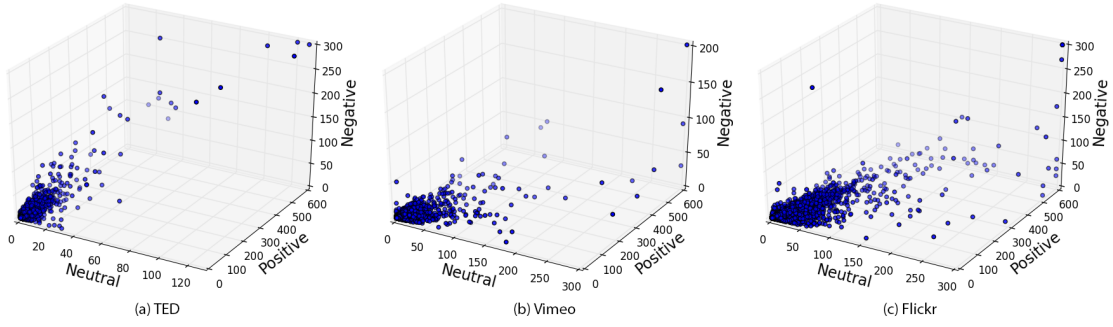
Figure 4.2: Three dimensional scatter plot of the number of positive, negative and neutral comments per user computed by the RB sentiment classifier. The opacity of the points indicates their depth in space. We can observe the dense areas and the spread over the axes of the sentiment distributions for each dataset. The dense areas for all datasets are concentrated in 0 to 200 of the positive axis, 0 to 100 of the neutral axis, and 0 to 50 of the negative axis; however, TED is more spread on the negative axis than Vimeo and Flickr.
