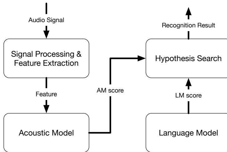
Figure 2.1: Architecture of ASR systems.
