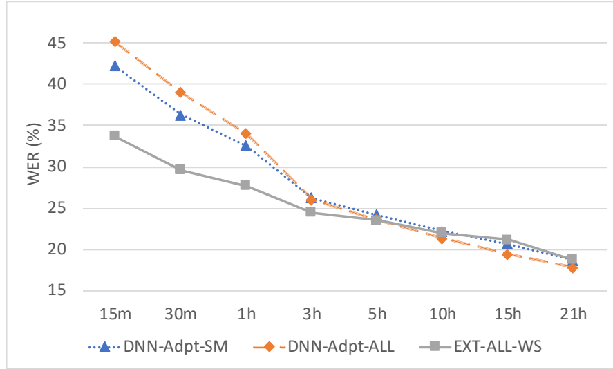
Figure 4.11: Comparison between CTC-based and DNN/HMM-based cross-lingual adaptation in WER(%). DNN-Adpt-SM denotes only updating the output layer of the DNN in the hybrid system. DNN-Adpt-ALL represents updating the whole network. EXT-ALL-WS is the CTC-based adaptation with the proposed parameter initialization.
