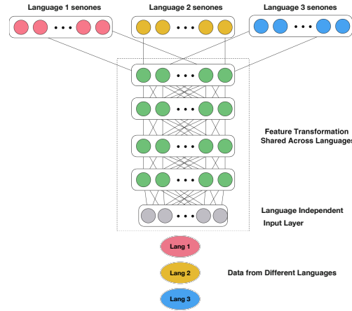
Figure 3.1: Architecture of the SHL-MDNN.
