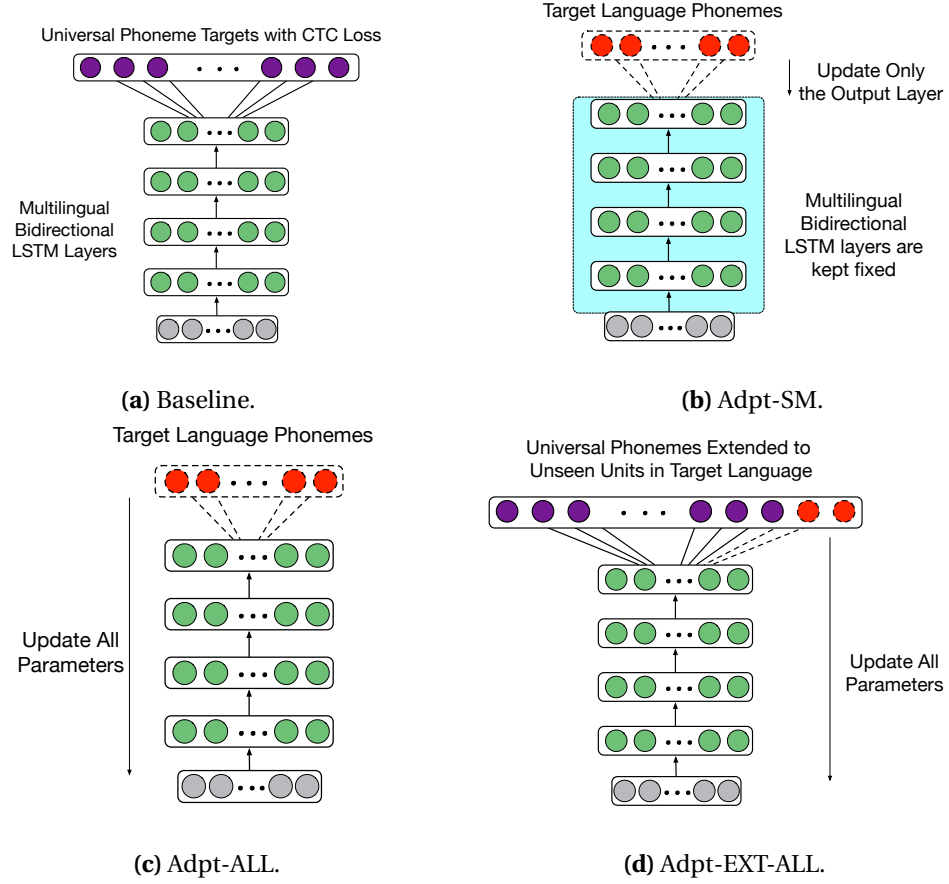
Figure 4.1: Approaches to adapt multilingual CTC model to the target language. (a) shows the baseline multilingual CTC model. In (b), a new softmax (SM) output layer replaces the multilingual targets. The hidden layers are fixed and only the output layer is re-estimated. We can also update all the parameters as shown in (c). In (d), the multilingual CTC model is extended to new phonemes by adding new connections. Adaptation is performed by updating all the parameters.
