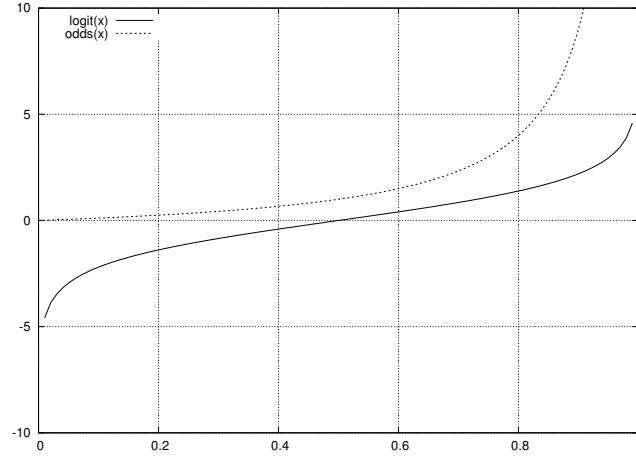
Figure 6.5: Logit and odds curves.
