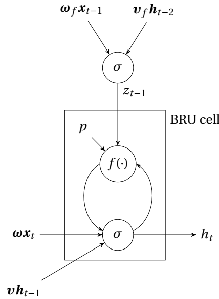
Figure 6.3: A Bayesian recurrent unit incorporating a probabilistic forget gate. An ad-hoc layer-wise and gate recurrence are retained.
