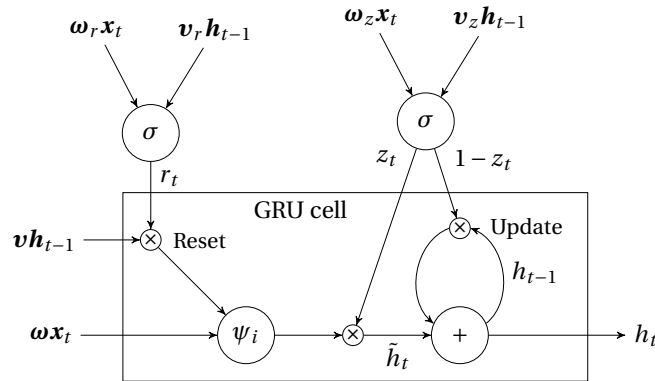
Figure 6.2: The gated recurrent unit of Cho et al. [2014]. As in the LSTM, the non-linearity \psi is usually tanh.
