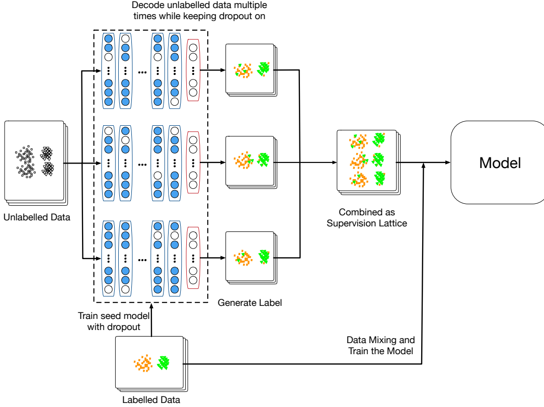
Figure 5.1: Flow-chart of the proposed method. Each network in the figure represents one network sample because of a different random selection of the active nodes. The white nodes denote that they are dropped out.
