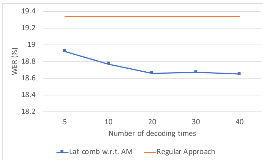
Figure 5.3: WER (%) of different semi-supervised training setup by varying the value of N . The dropout-based sampling is only applied on the acoustic model. The red line denotes the regular semi-supervised training approach [Manohar et al., 2018].
