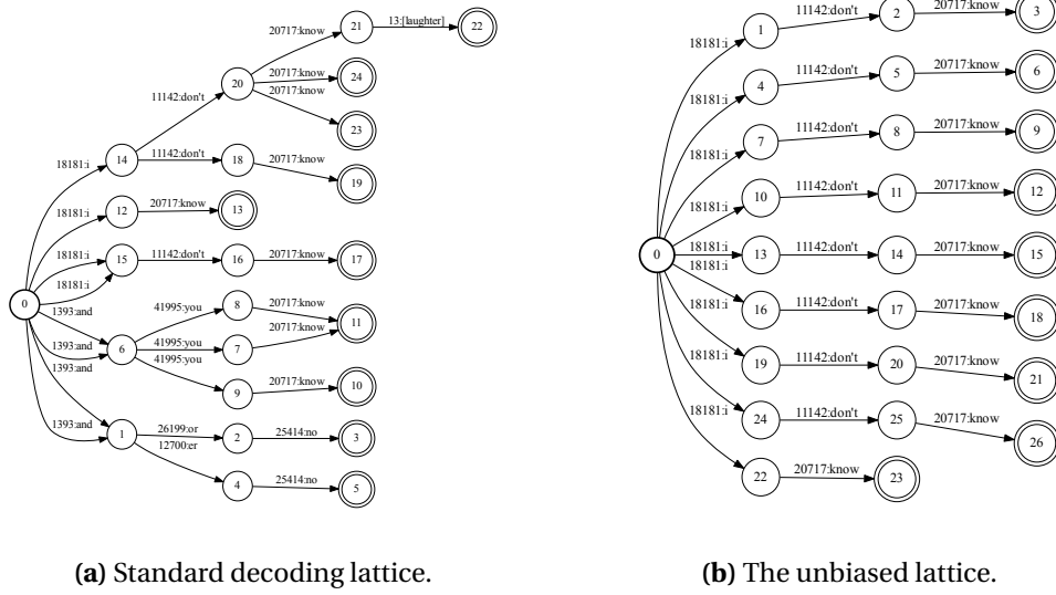
Figure 5.2: Lattices of a clearly spoken utterance. (a) represents the pruned decoding lattice from a dropout-off acoustic model. (b) denotes the unbiased lattice combined from multiple dropout decoding samples.
