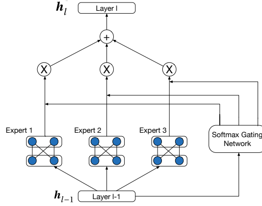
Figure 3.5: Architecture of MoE for one layer.
