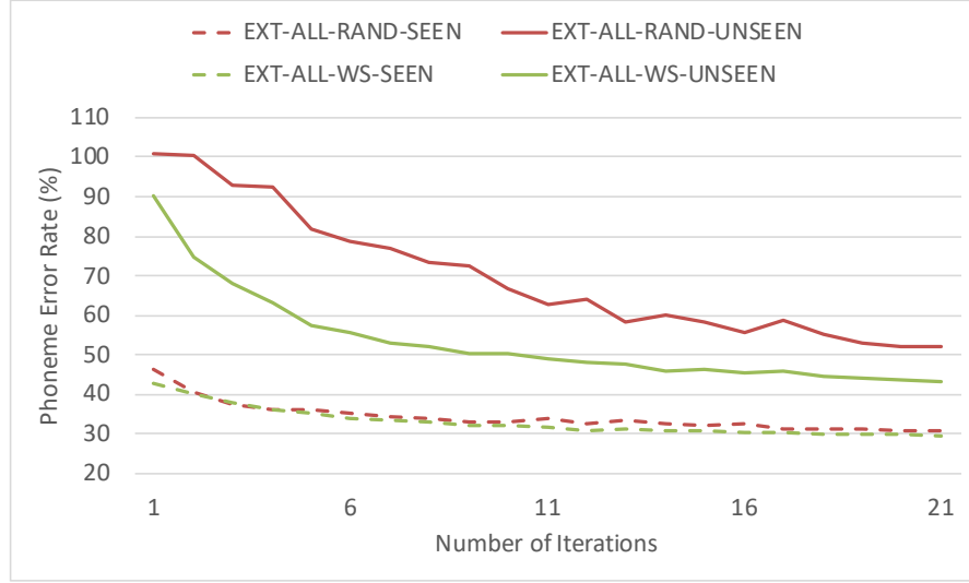
Figure 4.10: PERs (%) with respect to overlapped phonemes (SEEN) and new phonemes (UNSEEN) on PO development set. The adaptation was performed on 30 minutes data.
