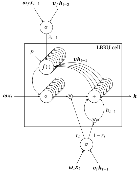
Figure 6.6: The layer-wise recursion with a forget gate and an input gate.
