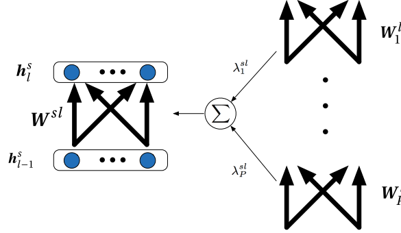
Figure 3.4: Architecture of CAT-DNN for one layer.
