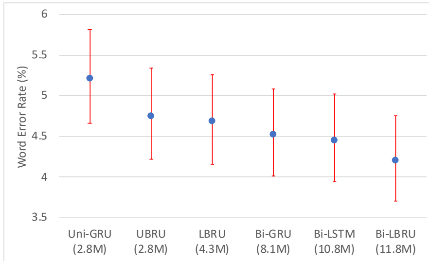
Figure 6.9: Word Error Rate (%) on WSJ for various RNN architectures. The numbers in the parentheses indicate the number of parameters each model contains. The error bars indicate equal-tailed 95% credible interval for a beta assumption for the error rate.
