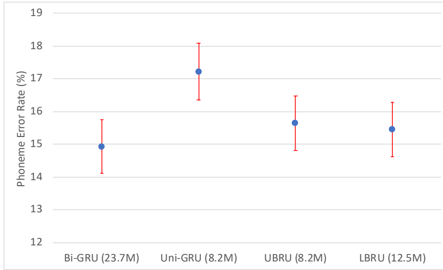
Figure 6.7: Phoneme Error Rate (%) on TIMIT for various RNN architectures. The numbers in the parentheses indicate the number of parameters each model contains. The error bars indicate equal-tailed 95% credible interval for a beta assumption for the error rate.
