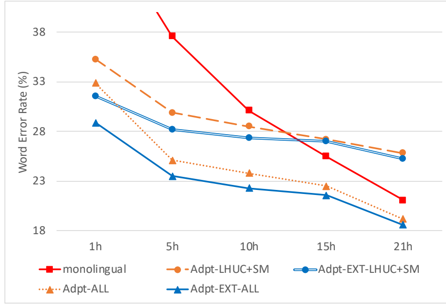
Figure 4.4: WERs (%) of different cross-lingual adaptation approaches. The WER of monolingual CTC model on 1 hour data is above 50% and exceeds the graph region. All models were trained with dropout.
