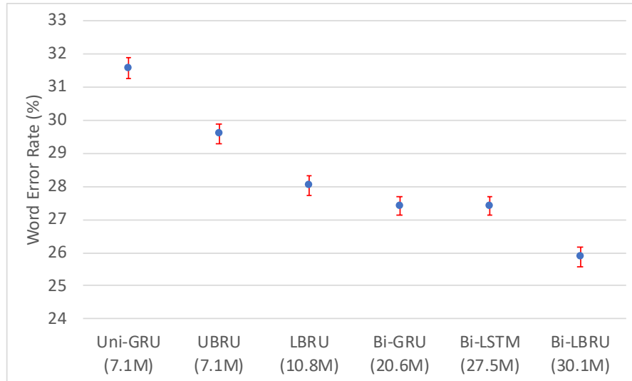
Figure 6.10: Word Error Rate (%) on AMI for various RNN architectures. The numbers in the parentheses indicate the number of parameters each model contains. The error bars indicate equal-tailed 95% credible interval for a beta assumption for the error rate.
