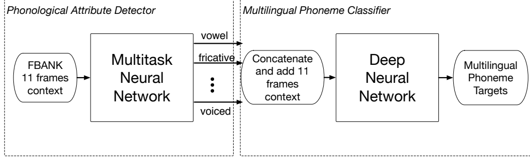
Figure 4.8: Architecture of the multilingual phoneme classifier using phonological features.
