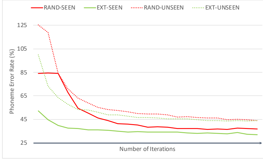
Figure 4.5: PERs (%) with respect to overlapped phonemes (SEEN) and new phonemes (UNSEEN) on PO development set. RAND denotes randomly initializing a new output layer before adaptation and EXT represents extending the multilingual output layer to the target language. The adaptation was performed by updating only the output layer and the LHUC layers on 1 hour data.
