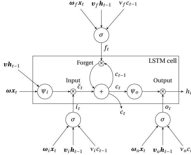
Figure 6.1: The long short term memory of Hochreiter and Schmidhuber [1997]. Non-linearities \psi are taken to be tanh.
