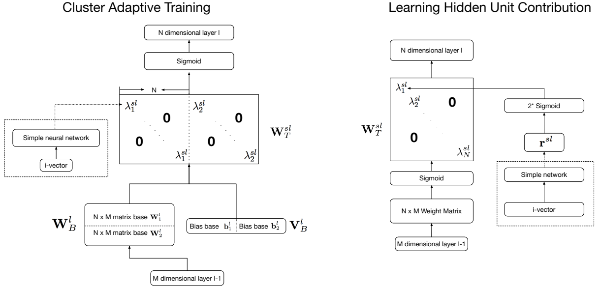
Figure 3.6: The common framework of CAT and LHUC. In CAT, an adaptation matrix \mathbf{W}_T^{sl} is inserted upon the concatenated weight bases \mathbf{W}_B^l and the bias. While in LHUC, a diagonal adaptation matrix is inserted above the Sigmoid activation.
