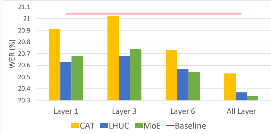
Figure 3.7: Comparison in WER(%) of LAT on different layers. The baseline is the IPA-based multilingual system.
