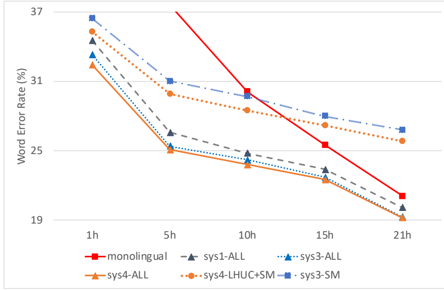
Figure 4.3: WERs (%) after cross-lingual adaptation of different multilingual models on various amounts of data. Dropout is applied in all systems. sys1-ALL denotes adapting all the parameters from sys1 . sys4-ALL is updating the whole network after removing the LHUC layers. sys4-LHUC+SM represents adapting only the Softmax output layer and the LHUC parameters from sys4 . sys3-SM is adapting only the output layer from sys3 .
