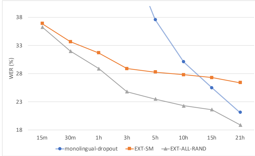
Figure 4.9: WERs (%) of different approaches in cross-lingual adaptation. The WERs of monolingual CTC models on less than 5 hours data are above 50% and exceed the graph region.
