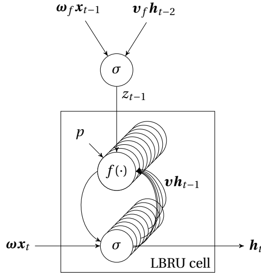
Figure 6.4: The layer-wise recursion with a forget gate.
