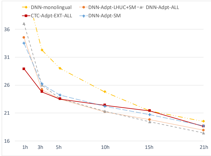
Figure 4.7: Comparison between CTC-based and DNN/HMM-based cross-lingual adaptation in WER(%). DNN-Adpt-ALL denotes updating all the parameters in DNN and DNN-Adpt-LHUC+SM represents updating the output softmax layer and the LHUC layers. DNN-Adpt-SM is only updating the output layer. The WER of monolingual DNN model on 1 hour data is above 40% and exceeds the graph region.
