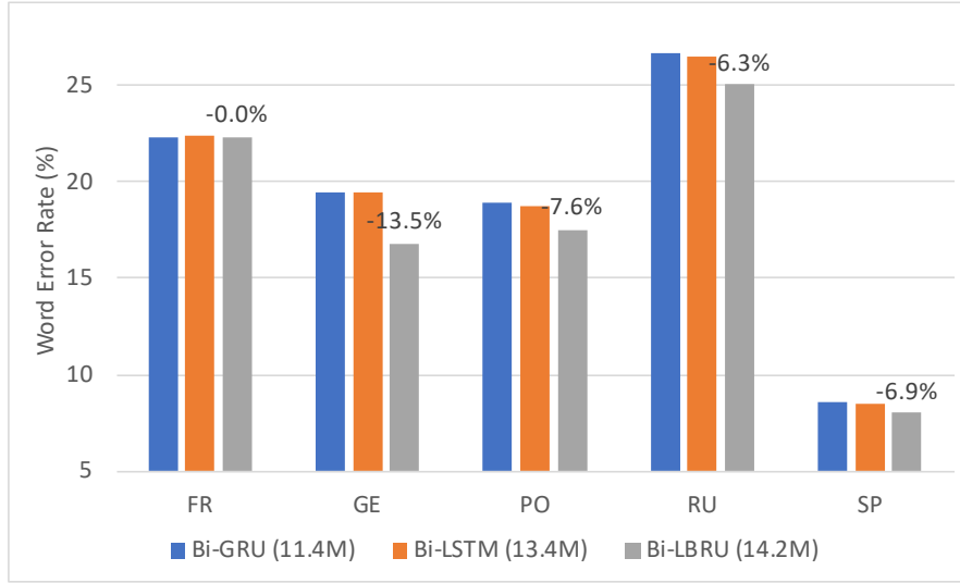
Figure 6.11: Word Error Rate (%) on the 5 selected languages from GlobalPhone for various RNN architectures. The numbers in the parentheses indicate the number of parameters each model contains. The numbers on top of the columns are the relative WER reduction of BRU compared with GRU architecture.
