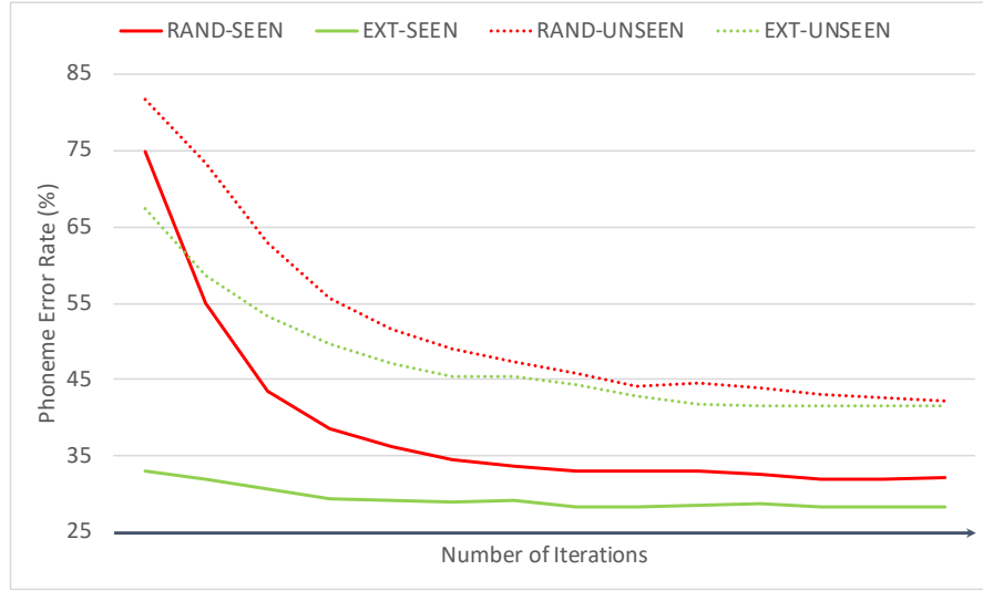
Figure 4.6: PERs (%) with respect to overlapped phonemes (SEEN) and new phonemes (UNSEEN) on PO development set. The adaptation was performed by updating the whole network on 1 hour data.
