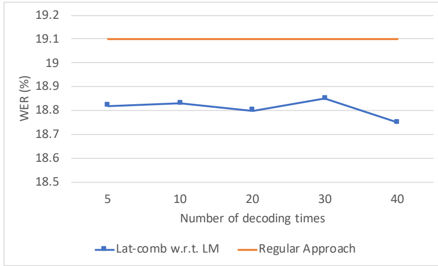
Figure 5.4: WER (%) of different semi-supervised training setup by varying the value of N . The dropout-based sampling is only applied on the language model. The red line denotes the regular semi-supervised training approach Manohar et al. [2018] where the supervision lattices of unsupervised data were also re-scored using NN LM.
