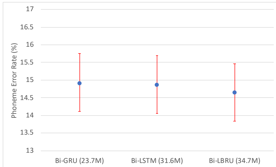
Figure 6.8: Phoneme Error Rate (%) on TIMIT for various RNN architectures. The numbers in the parentheses indicate the number of parameters each model contains. The error bars indicate equal-tailed 95% credible interval for a beta assumption for the error rate.
