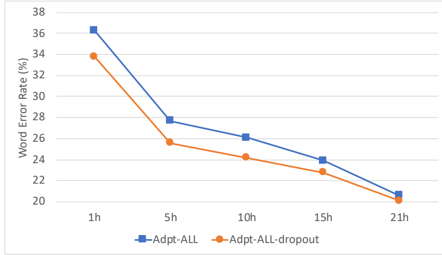
Figure 4.2: WERs (%) after cross-lingual adaptation with or without dropout.
