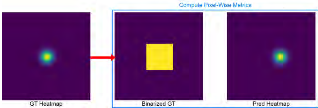
Figure 4.2: The heatmap metric for gaze following proposed by Chong et al. (2020b), and by Li et al. (2018) for egocentric gaze estimation, compares the predicted heatmap to a binarized ground truth heatmap at the pixel level. However, the binarization threshold is arbitrary and, in the case of Chong et al. (2020b), results in an overly large positive region. This setup also penalizes multimodal predictions when they fall outside this region. Moreover, the metric is difficult to interpret and lacks a clear correspondence to meaningful spatial or semantic error, which limits its utility. For these reasons, we do not compute this metric in our later works.
