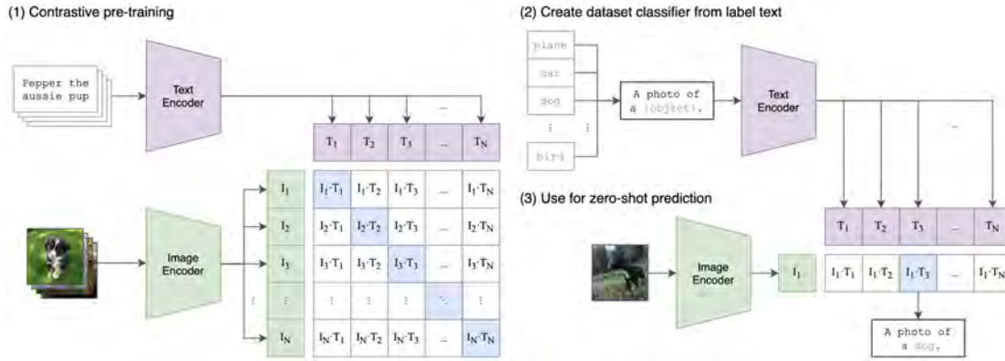
Figure 2.9: CLIP (Radford et al., 2021) uses contrastive training to align image and text embeddings (1). At inference time, zero-shot classification is enabled by constructing a set of text prompts (2), computing their embeddings, and selecting the one that has the highest similarity with the image embedding (3).
