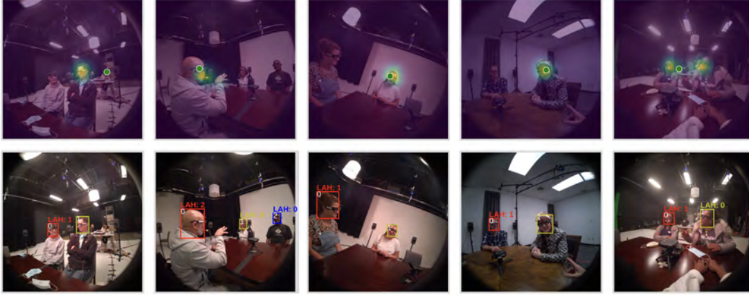
Figure 8.4: Qualitative results on RLR-CHAT for egocentric (top) and exocentric (bottom) gaze prediction using the encoder initialized with our Explicit Matching based self-supervised approach. The predicted egocentric gaze heatmap is overlaid on the image, with the ground truth target marked by a green dot. Predicted exocentric gaze targets are indicated by the person ID following the 'LAH' prefix.
