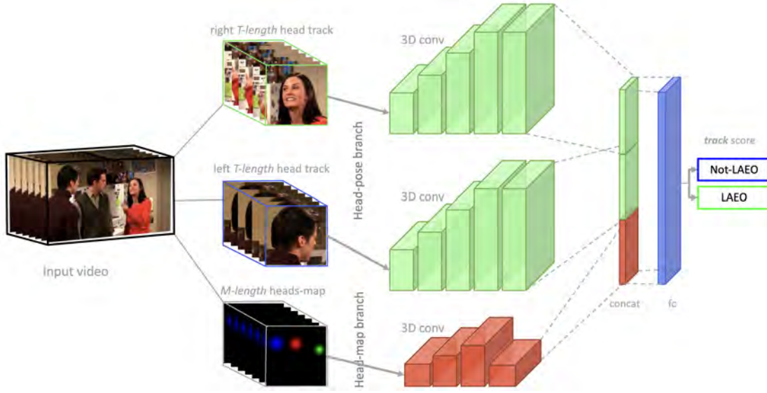
Figure 2.5: Several prior works for social gaze estimation proposed task-specific architectures, such as this one from Marín-Jiménez et al. (2021) for LAEO. It also only supports processing pairs of people, requiring multiple forward passes for all pairs of people in the scene.
