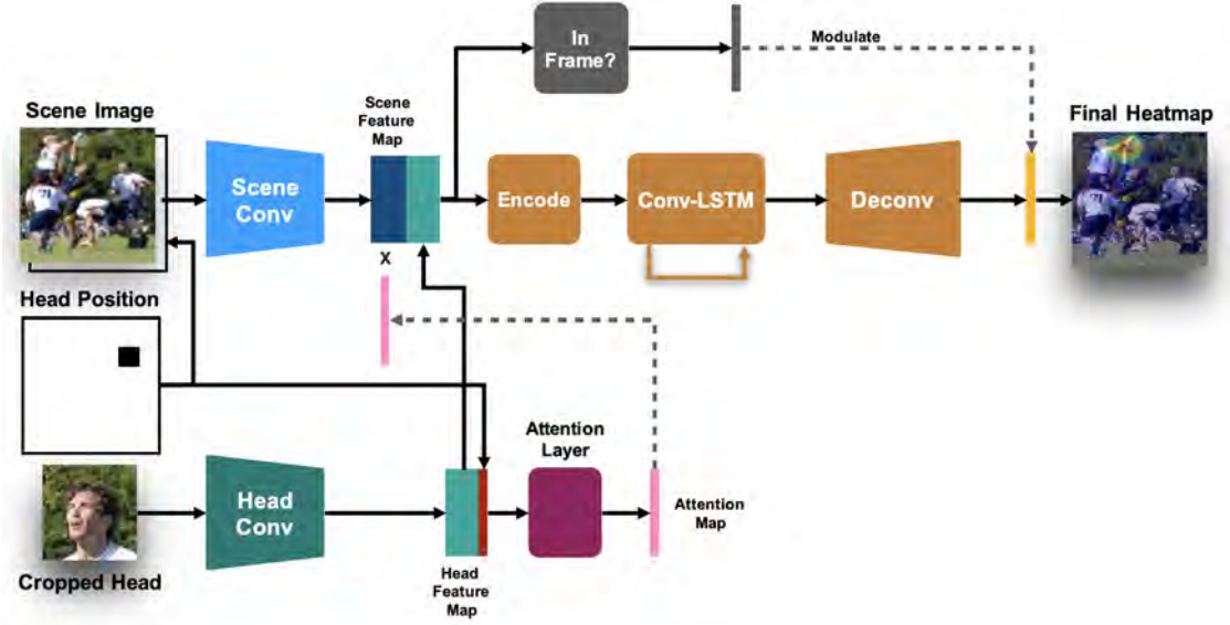
Figure 2.4: Chong et al. (2020b) were the first to explore the use of temporal information for enhancing gaze following by applying an LSTM over bottleneck features from the scene and head branches. However, this approach yielded only marginal improvements compared to their static version.
