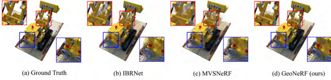
Figure 3.1: Our generalizable GeoNeRF model infers complex geometries of objects in a novel scene without per-scene optimization and synthesizes novel images of higher quality than the existing works: IBRNet (Wang et al., 2021b) and MVSNeRF (Chen et al., 2021).
