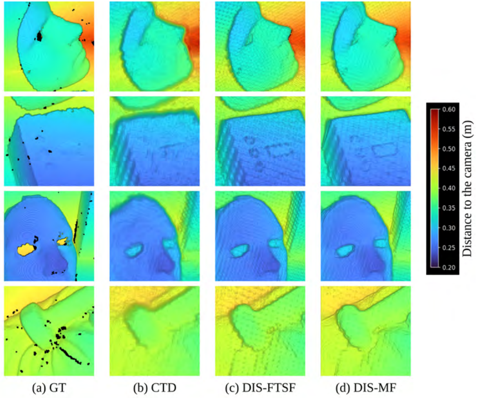
Figure 2.16: Qualitative analysis of the depth maps rendered in OpenGL (Shreiner et al., 2013) and presented in the Turbo color map (Mikhailov, 2019). Samples are taken from the real dataset. This analysis shows how our models outperform the state-of-the-art model, CTD (Riegler et al., 2019), in preserving details of the 3D objects and producing sharp edges. It is noticeable that in some regions ( e.g. , the top edge of the box in the second row in column (a)), ground truth depths are noisy, and it is due to the limitations of the 3D scanner we used to capture ground truth depths. Since all evaluated methods are self-supervised, their performances are not affected by the ground truth noise. (a) Ground truth depth map. (b) CTD (Riegler et al., 2019). (c) Our DIS-FTSF model. (d) Our DIS-MF model. For further information about 3D rendering of depth maps, refer to Section 2.8.6. The color bar represents depth values in meters.
