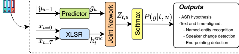
Figure 6.7: a) Proposed unified token augmentation protocol for SCD, ENDP, and NER. b) TokenVerse unifies multiple speech and NLP tasks (e.g., T1+T2+T3 ) in a single model within the neural Transducer framework.
