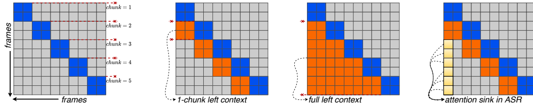
Figure 4.7: Masking strategies for streaming XLSR-Transducer. Multi-chunk training allows decoding with variable chunk size (blue) and left context (orange). Each square denotes “n” frames. Attention sink (yellow) allows context from the first n frames. Our results show that attention sink frames offer a better trade-off w.r.t increasing left context alone , leading to lower WERs.
