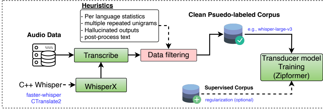
Efficient pseudo-labeling and training with foundational speech model
