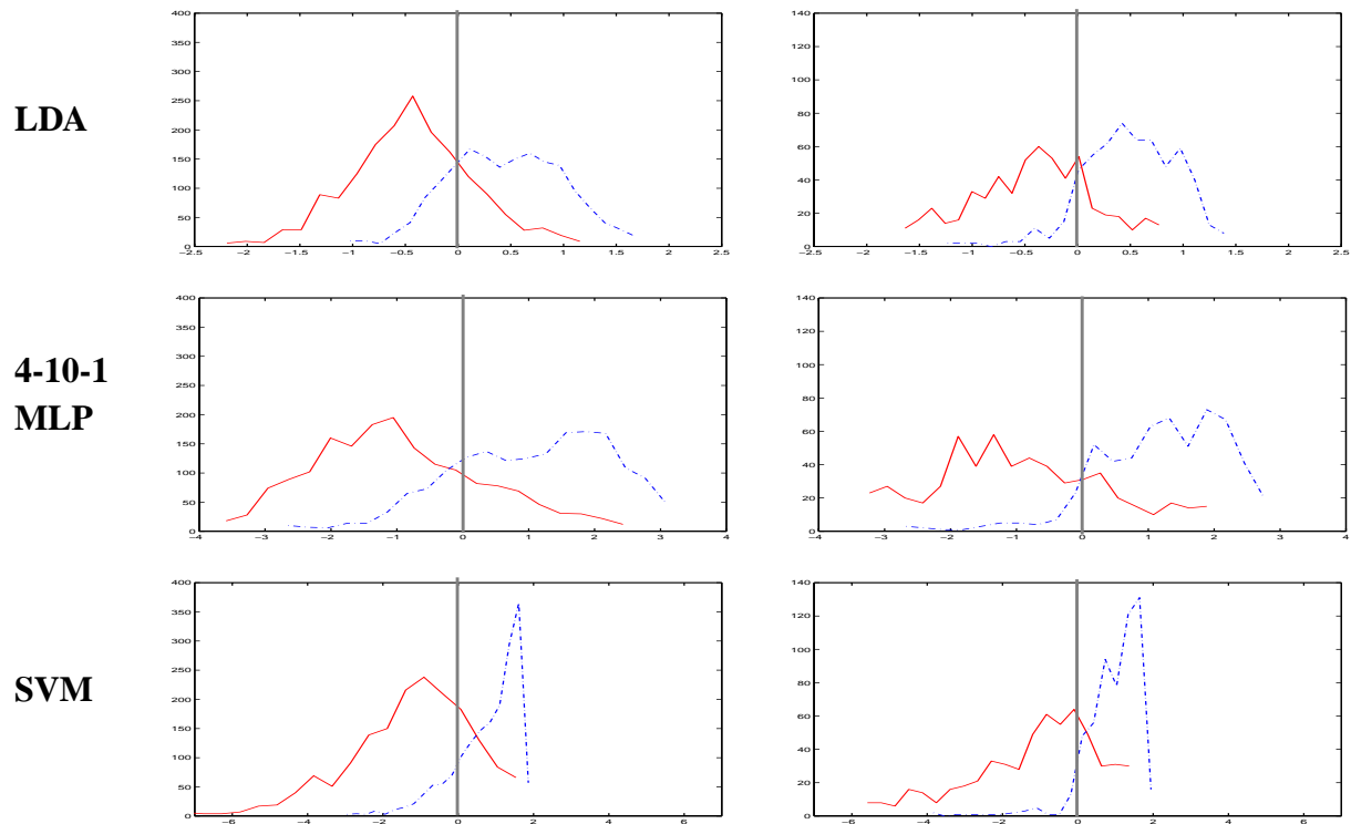
Figure 4. Histograms of projected training data (left) and corresponding test data (right) using LDA (top), MLP (centre) and SVM (bottom) for one training/test subset for one subject (k4). “Left” data = solid, “right” data = dashed. Training set is parts 1,2,3, test set is part 5. Respective test data %correct scores for this example are 83.9, 83.0 and 82.9 respectively (MLP values are pre-squashed MLP class probability outputs).
