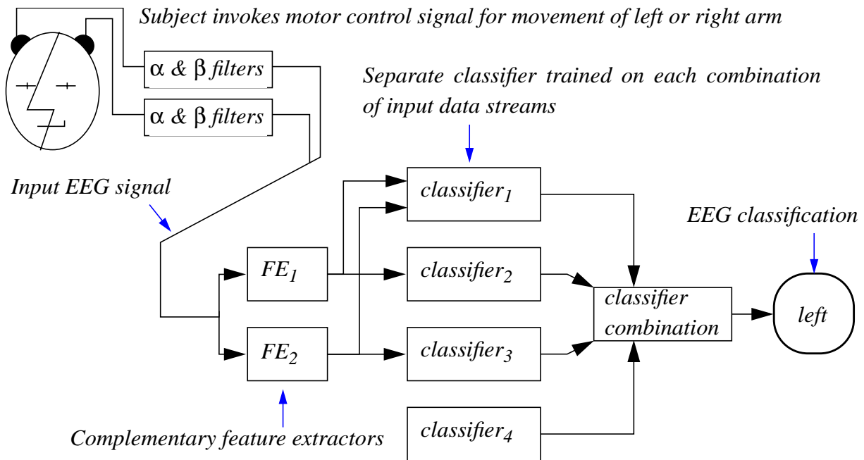
Figure 1. Multi-stream single frame EEG decoder. Two or more types of feature vector are extracted from a short term EEG sample. In training a separate classifier (for example, an MLP) is trained on every combination of these feature vectors. In recognition the class probabilities from each classifier are combined by some rule (such as MAP) taking into account the relative reliability of each classifier.
