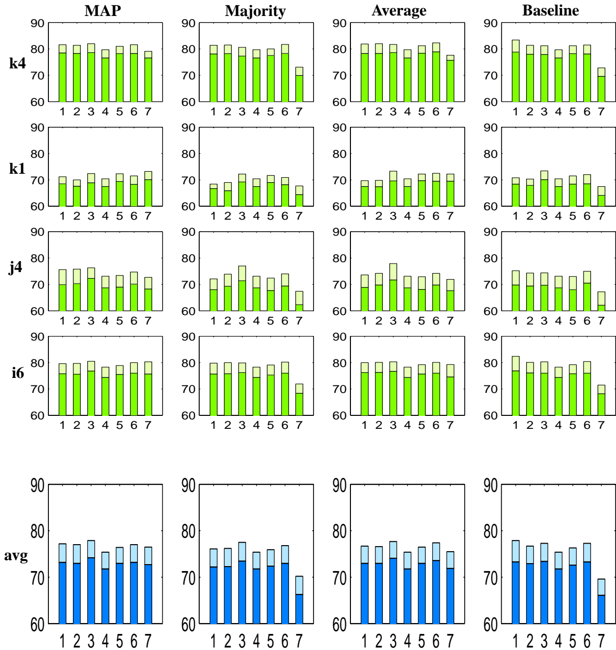
Figure 5. Comparison of multi-classifier combination %accuracy (columns 1-3) with single classifier baseline. Percentage accuracy results are shown for seven different classifier types (1:LDA, 2:MLP, 3:SVM, 4:GMC, 1-mix, 5:GMC:, 3-mix, 6:MLP with VSE, 7:SVM with VSE). Each system first performs independent classification with data from each possible selection of 1 or more coefficients from the 4 dimension the data vector. Separate classifiers are then combined using either the MAP, “majority” or “average” rule. Rows 1 to 4 give results for each subject. Row 5 shows average accuracy results over all subjects.
