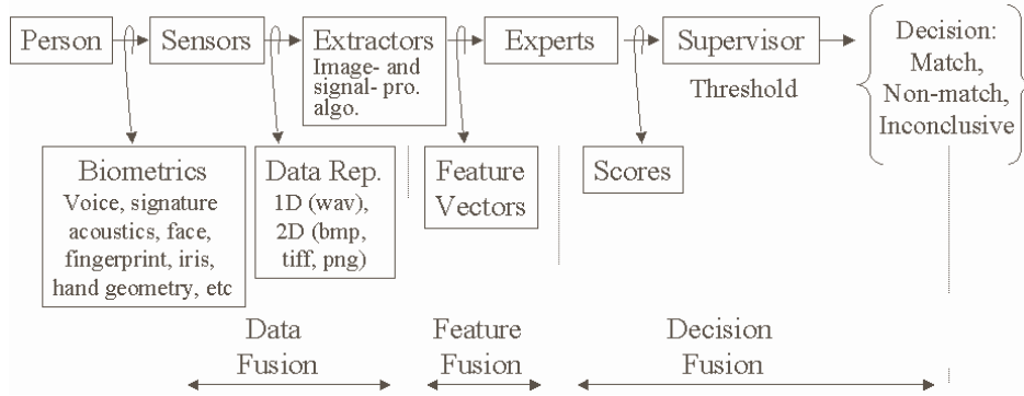
Figure 1: A generic biometric taxonomy and fusion scheme
