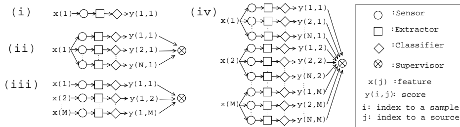
Figure 2: (i) Single-sample single-source, (ii) multi-sample single-source, (iii) single-sample multi-source and (iv) multi-sample multi-source biometric model. x(j) and y(i,j) are equivalent to \mathbf{x}_j and y_{i,j} in text respectively.
