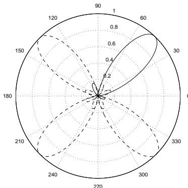
Figure 3: Microphone array directivity patterns at 1000 Hz (speaker 1 direction in bold)
