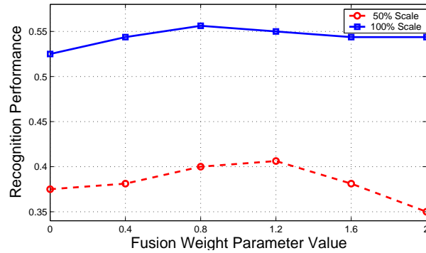
Figure 3: Fusion weight training curves.
