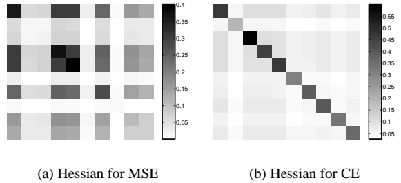
Fig. 1. Description of the Hessian matrix obtained with an MLP trained with the MSE criterion in (a) and with the CE criterion in (b). The Hessian has been averaged over all the examples. MLPs have 10 hidden units. Each block corresponds to a pair of hidden units, and is represented by its spectral norm. Results on the Forest dataset, with 10,000 training examples, after 5 iterations.
