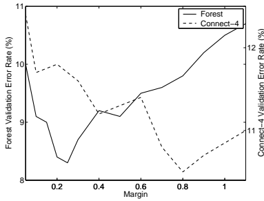
Fig. 2. Evolution of the validation error with respect to the margin for an MLP with outputs weights \alpha fixed to 1. Results on Forest dataset.
