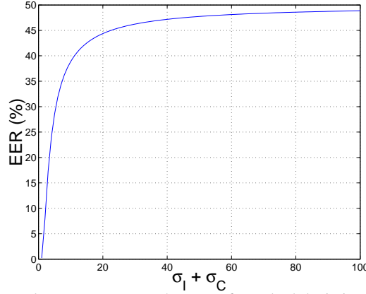
Fig. 2. Equal error rate versus the sum of standard deviations of client and impostor scores
