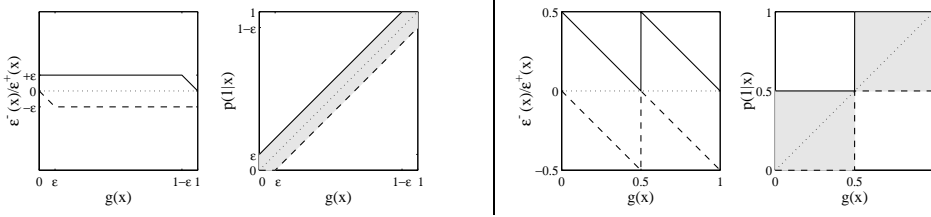
Figure 1: Two examples of \epsilon^-(\mathbf{x}) (dashed) and \epsilon^+(\mathbf{x}) (plain) vs. g(\mathbf{x}) and resulting \epsilon -tube of possible values for the estimate of P(Y = 1|X = \mathbf{x}) (gray zone) vs. g(\mathbf{x}) .
