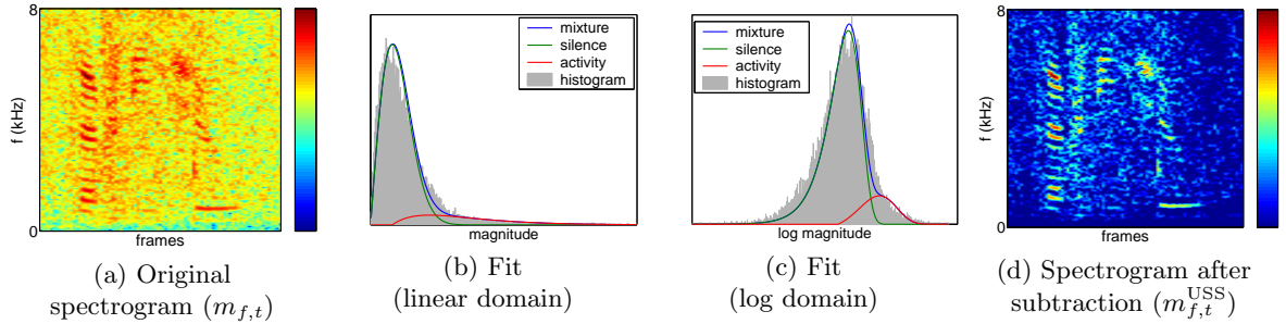
Figure 2: Example of fit of the 2-mixture model on noisy data taken from the OGI Numbers 95 database (Factory 0dB condition). All plots show magnitude data in the frequency domain. On spectrogram plots (a) and (d), the largest magnitudes are red, the smallest magnitudes are blue.
