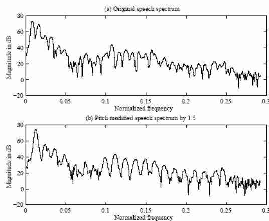
Figure 33 : Original and modified spectrum by \beta = 1.5
