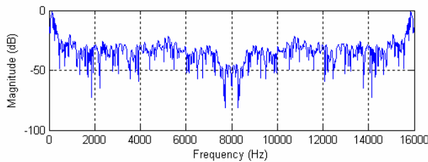
Figure 6 : Spectral frame synthesized by LP
