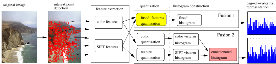
Figure 1: Schematic representation of our system and of the two alternative fusion approaches: fusion between texture and color information is done either at the feature level before quantization (yellow box) or at the bag-of-visterm level (pink box).
