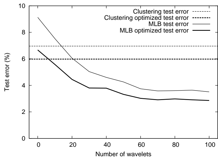
Figure 4: Test error rates with and without pose optimization as a function of the number of Haar wavelets per feature in the hidden layer. Not shown here is the error rate of 1.46% with 1,000 weak learners in the output layer, 50 wavelets in the hidden layer and tilt optimization (1.87% without).
