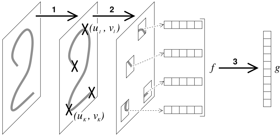
Figure 1: The classification is composed of three steps: (1) on the input image I a fixed number K of points of interest (u_1, v_1), \dots, (u_K, v_K) are tagged on the maxima of a difference of Gaussians, (2) a feature vector of size D is computed for each of these points of interest, as a function of the \Delta \times \Delta neighborhood of each points, resulting in a vector f(I) of dimension D K , (3) one response g_c is computed for each of the C classes as a function of both the locations of the points of interest and the feature vectors.
