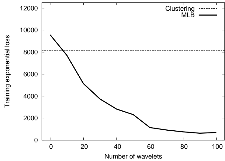
Figure 3: Exponential loss during training as a function of the number of Haar wavelets used in the hidden layer for the Multi-Layer Boosting (MLB) with 100 weak learners per class in the output layer.
