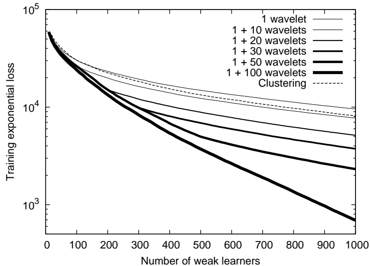
Figure 2: Exponential loss as a function of the total number of weak learners in the output layer when the wavelets in the hidden layer are added from the first step of learning.
