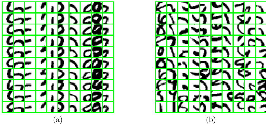
Figure 5: These figure show for each of the D = 32 feature component the eight \Delta \times \Delta subimages with the highest score. Figure (a) corresponds to the EM clustering and (b) to the multi-layer boosting with 100 wavelets. As observed for multi-layer perceptrons, the features obtained by supervised learning are less consistent geometrically than those learnt by unsupervised learning.
