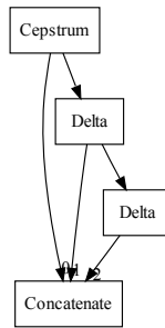
Figure 2: Tracter sub-graph to append dynamic features.
