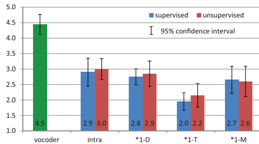
Fig. 2. Naturalness score (speaker H )
