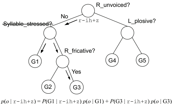
Fig. 1. An example of decision tree marginalization, showing how a new recognition model “r-ih+z” is derived from a decision tree of a speech synthesis system (“L_” / “R_”: left/right phone; “G?”: clustered state emission distribution PDFs)
