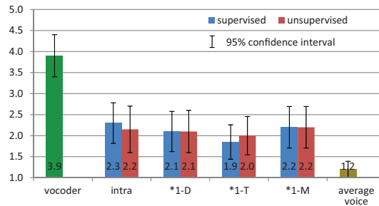
Fig. 4. Similarity score (Mandarin reference uttered by speaker H )
