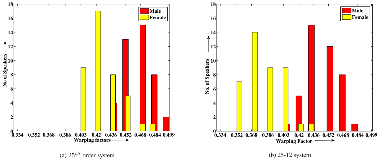
Fig. 2: Warping factors estimated from 25 th order features. The 25-12 system initializes the features with the warping factors estimated from 12 th order features. Both graphs have same range for X-axis.
