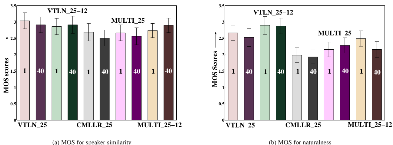
Fig. 5: MOS for naturalness and speaker similarity of synthesized speech. 1 and 40 represents number of adaptation sentences. MULTI represents the combination of VTLN and CMLLR adaptation techniques.
