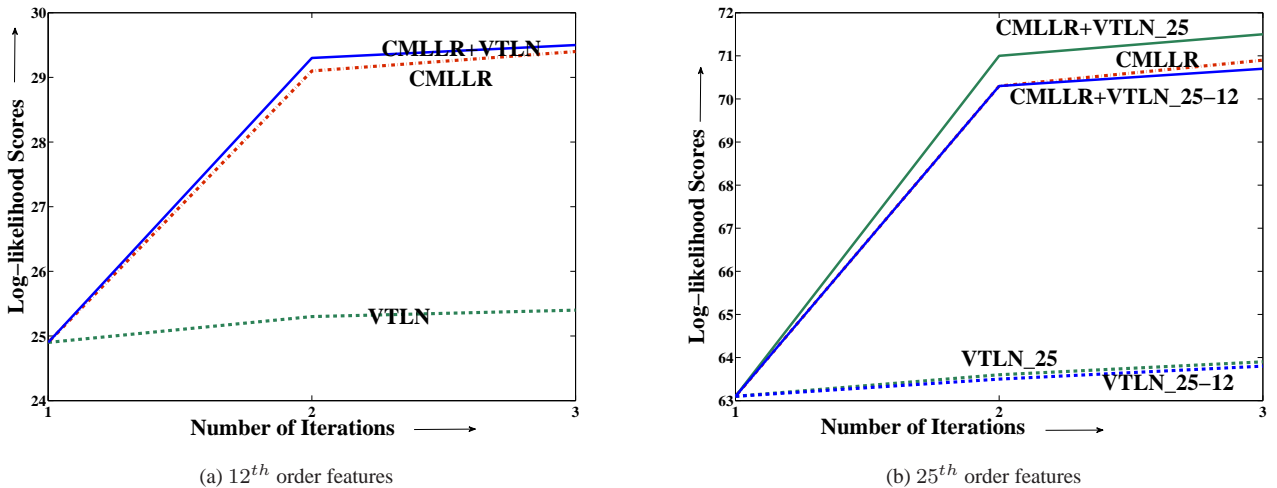
Fig. 3: Log-likelihood scores during training.
