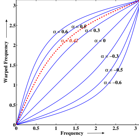
Fig. 1: Bilinear Transform
