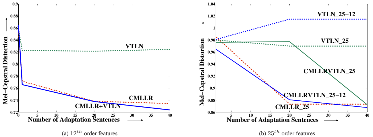
Fig. 4: Mel-Cepstral Distortion for synthesized speech.
