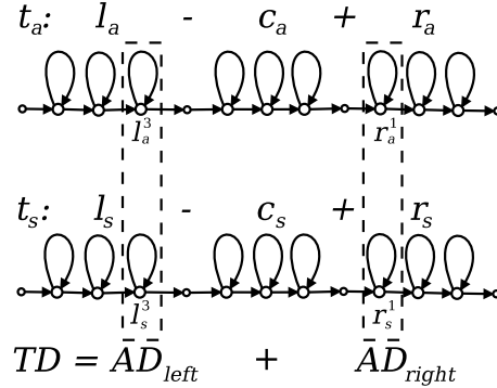
Figure 1: Acoustic triphone distance \operatorname{TD}(t_a, t_s) calculation based on acoustic left and right contextual distances, keeping the same center phonemes c_a = c_s .
