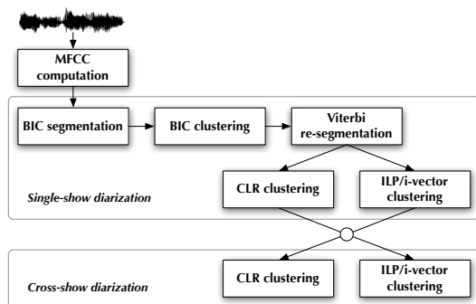
Figure 1: Diarization steps
