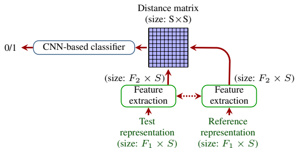
Fig. 1: Block diagram of the proposed pairwise distance-based dysarthric speech detection CNN. The two feature extraction blocks share the same set of parameters.
