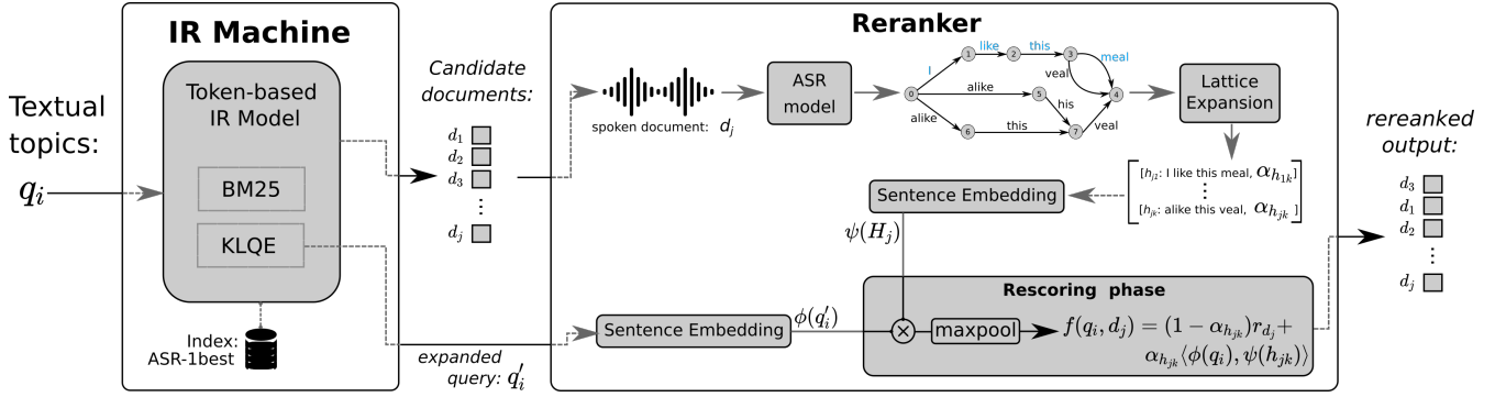
Figure 1: General overview of the proposed multi-stage retrieval architecture based on expanded lattice embeddings.
